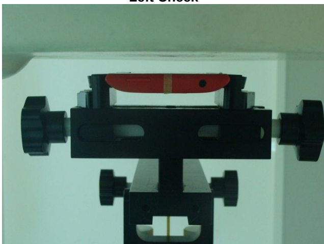
Front of the DUT with Phantom 1 cm Gap (DUT without Headset)
