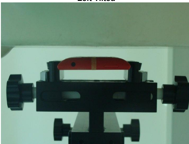
Back of the DUT with Phantom 1 cm Gap (DUT without Headset)
