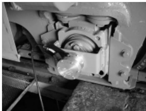
Figure 1.3-10 Axle Generator
