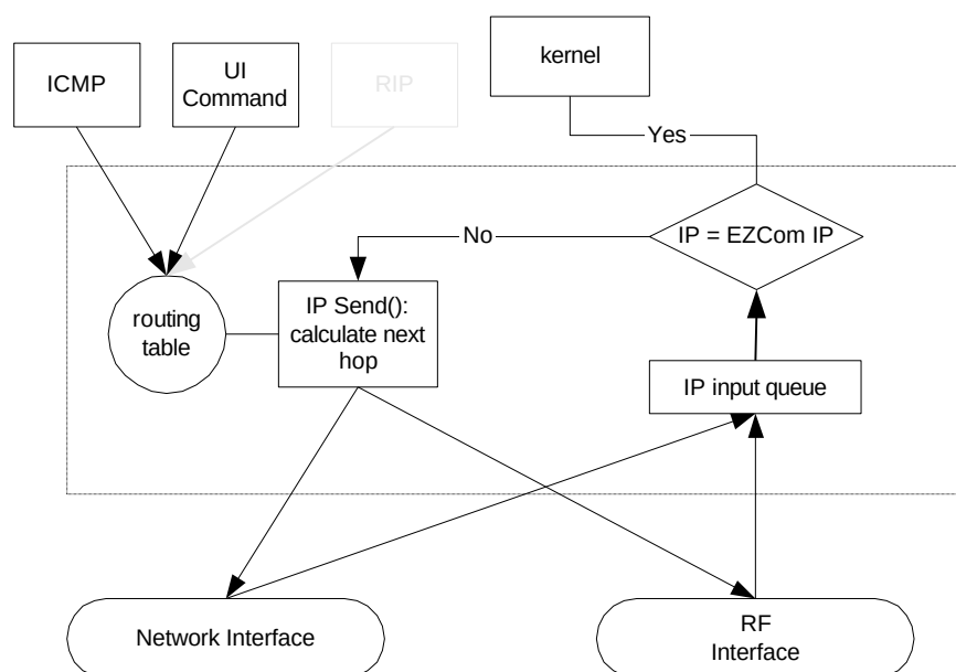
Figure 18, EZCom-IP Routing Mechanism
