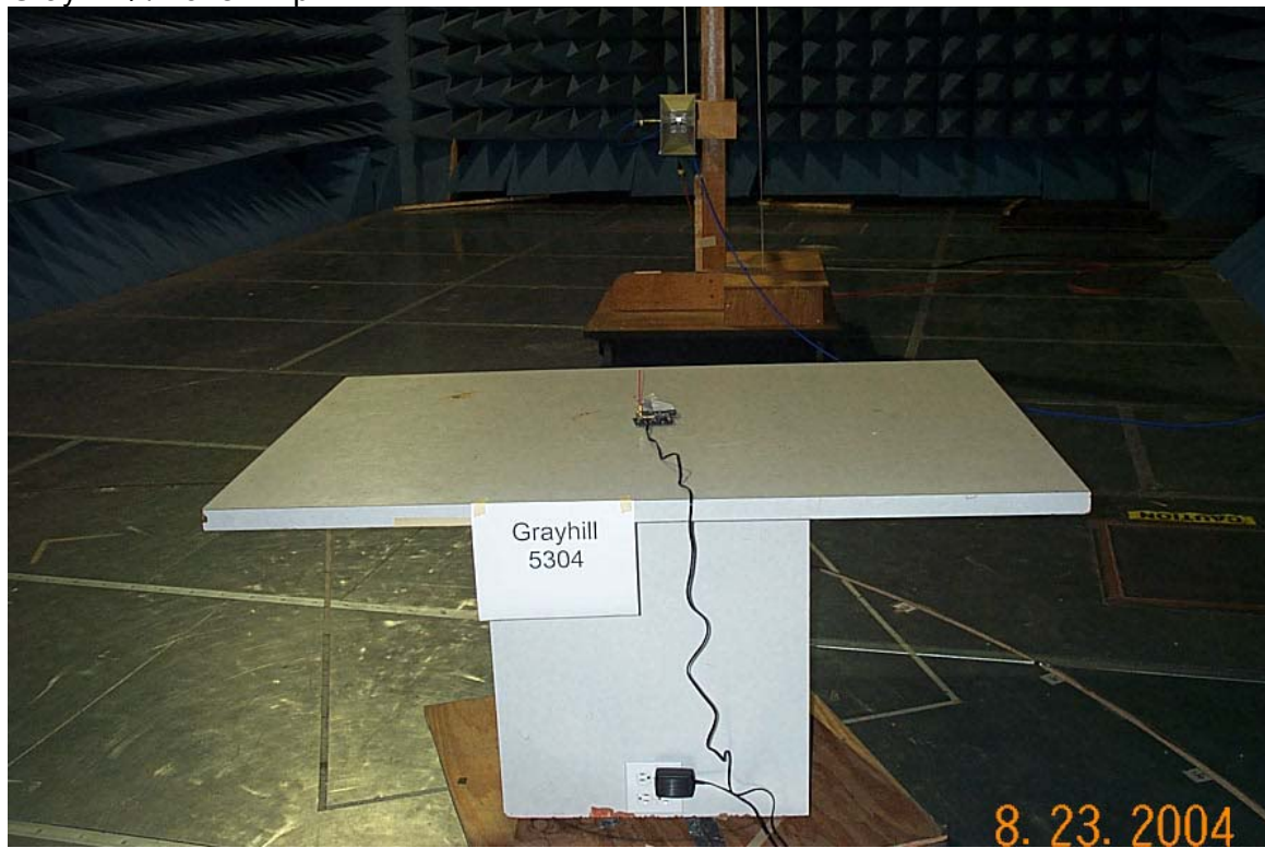
Grayhill ¼ wave whip
