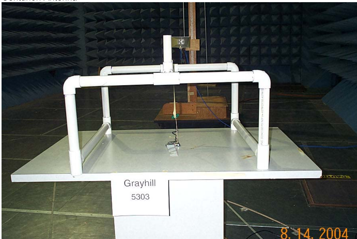
Centurion Antenna
