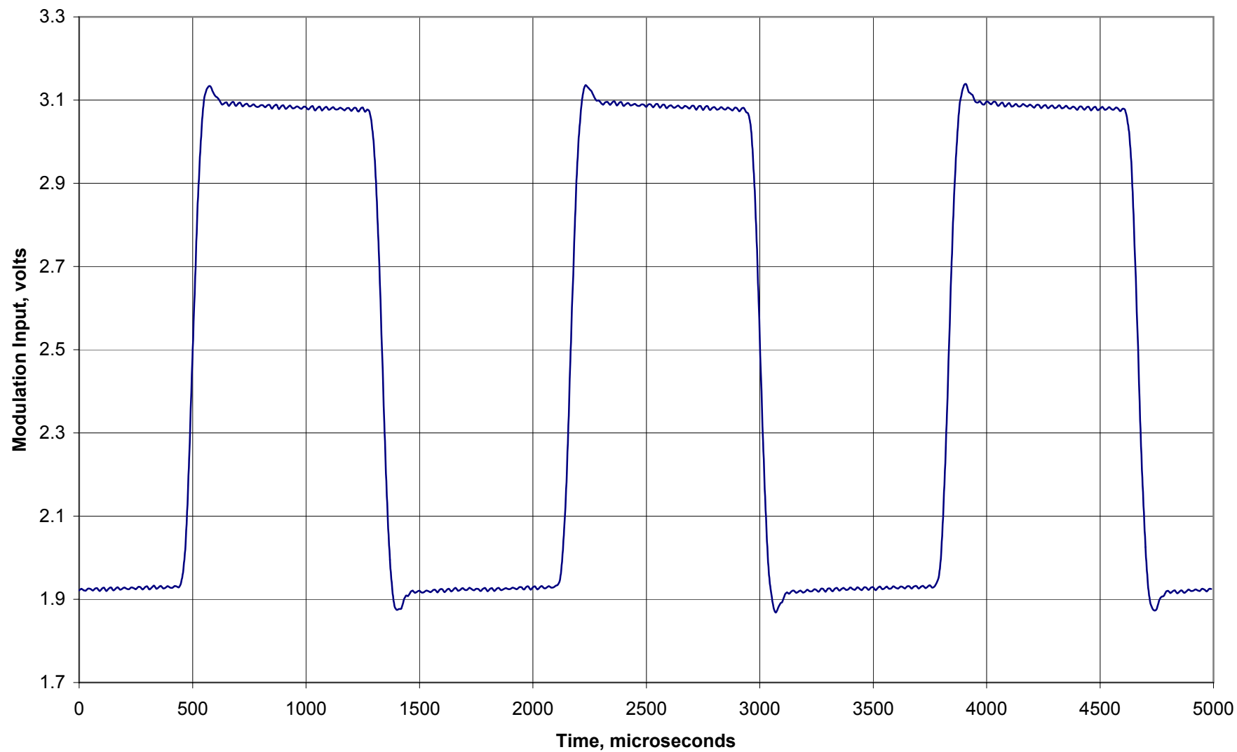
Modulation Input to DM-3473 Transceiver, Transmit Mode
