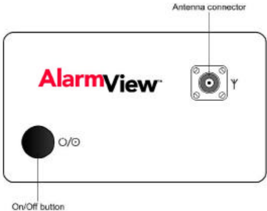
Transmitter Top View
