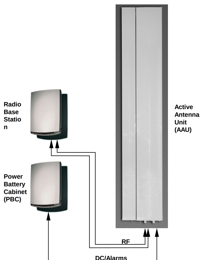
Figure 1 Active Antenna and Related Equipment
