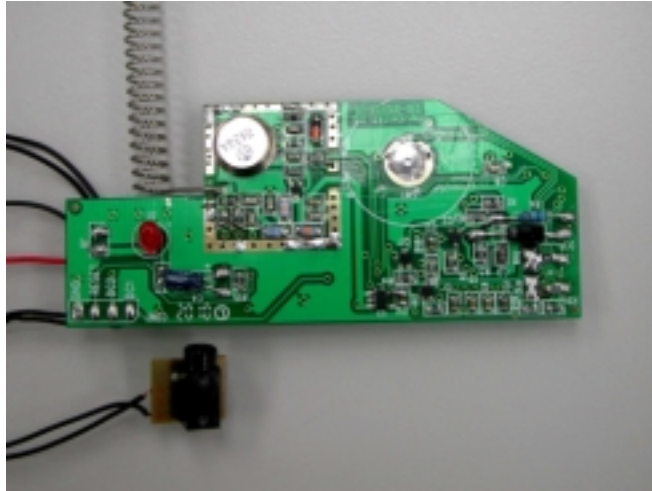
Internal Photo – 4
