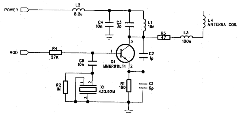
UHF TRANSMITTER
