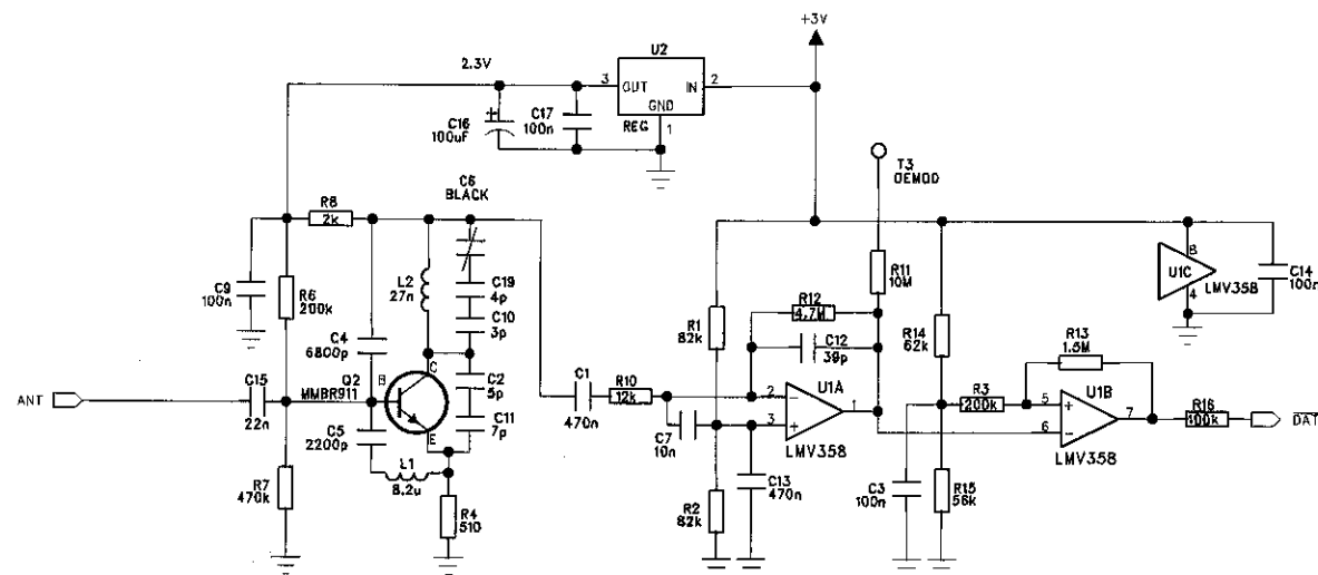
UHF RECEIVER
