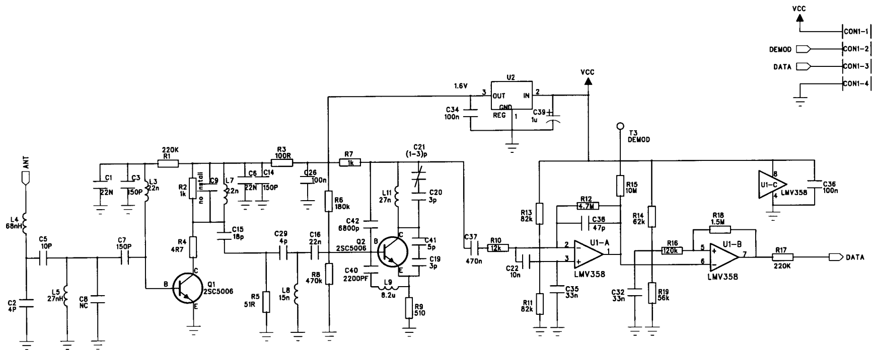
UHF RECEIVER
