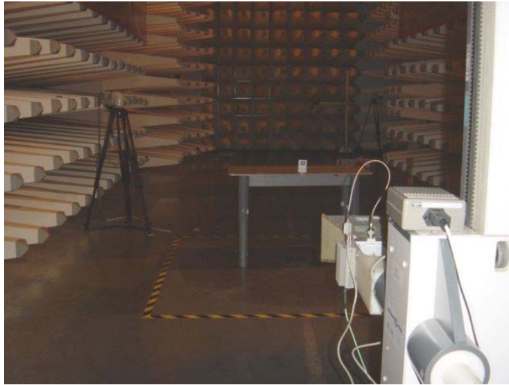
Set-up for Radiation Emission ( Transmitter)
