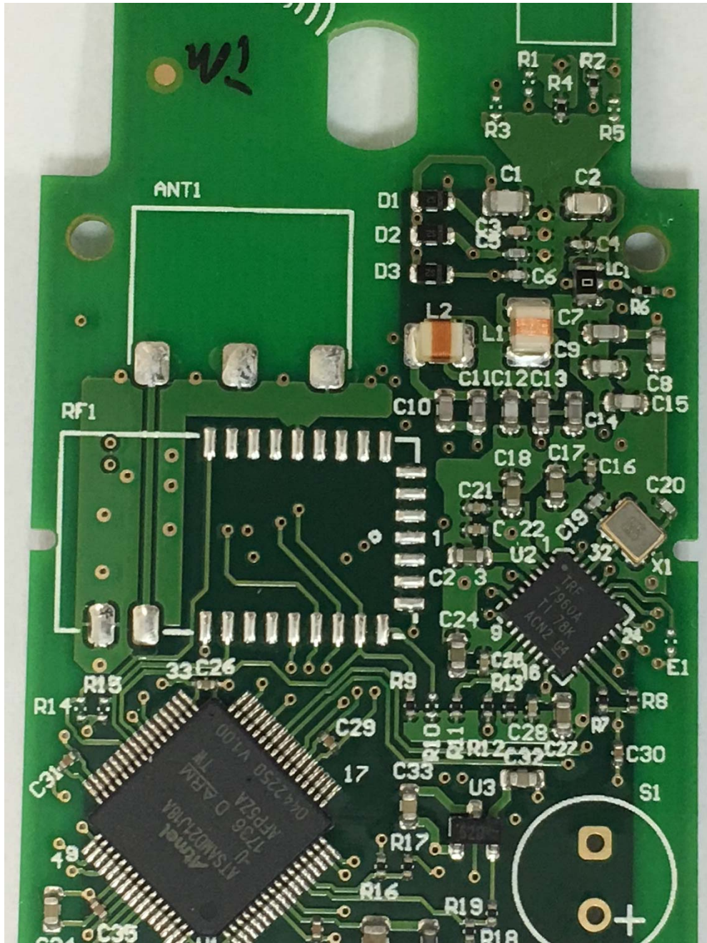
EUT TOP (NO SHIELD CLOSE UP)
