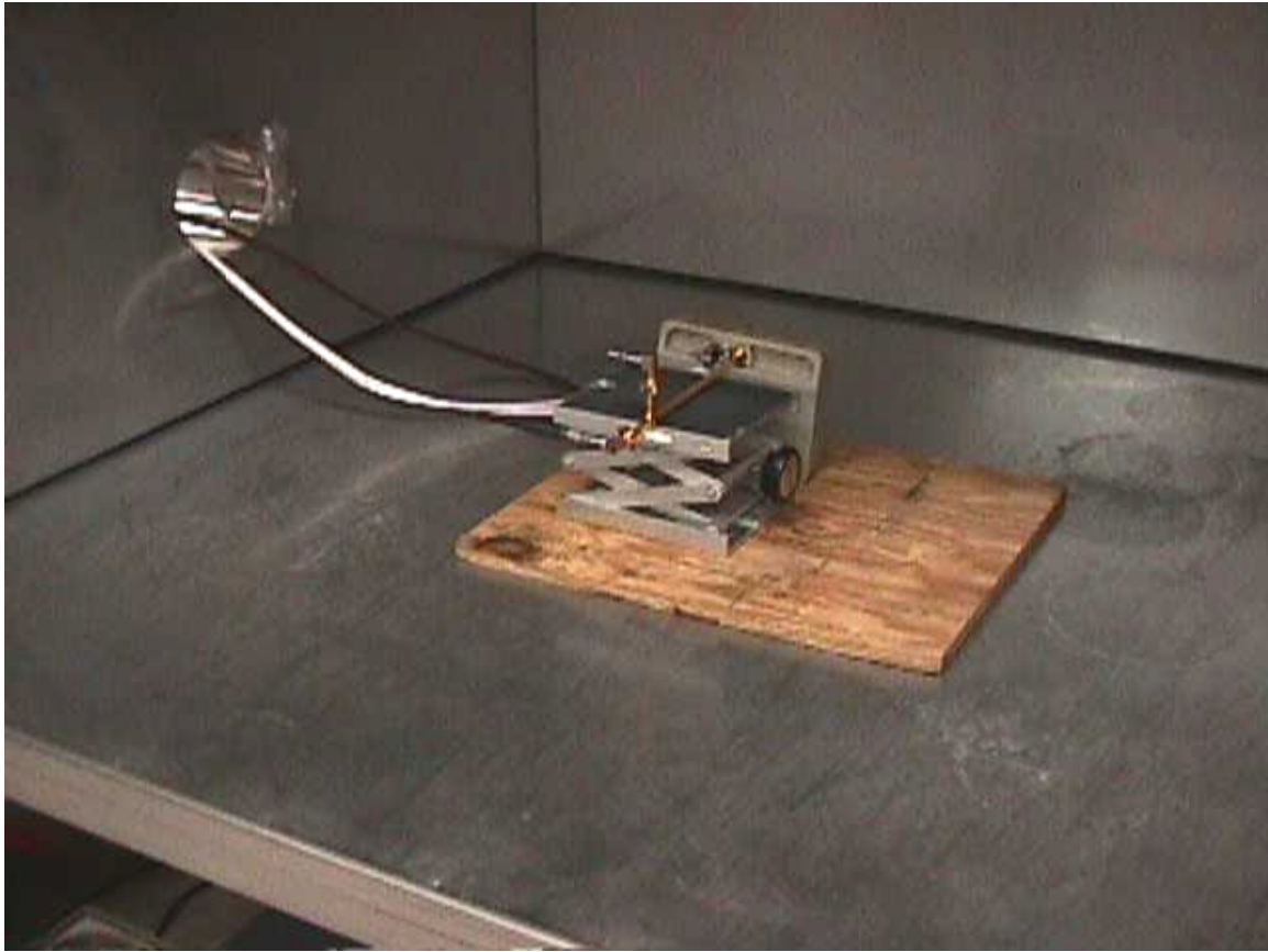
Figure 7-5 Setup for frequency stability measurements - chamber
