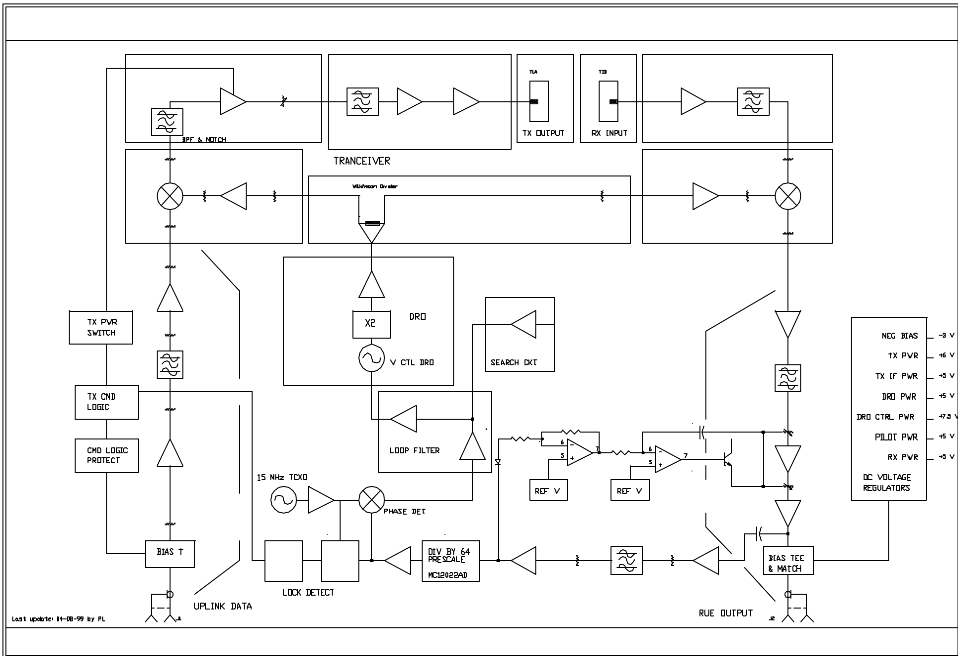
Figure 4-1 CPE ROOF UNIT BLOCK DIAGRAM
