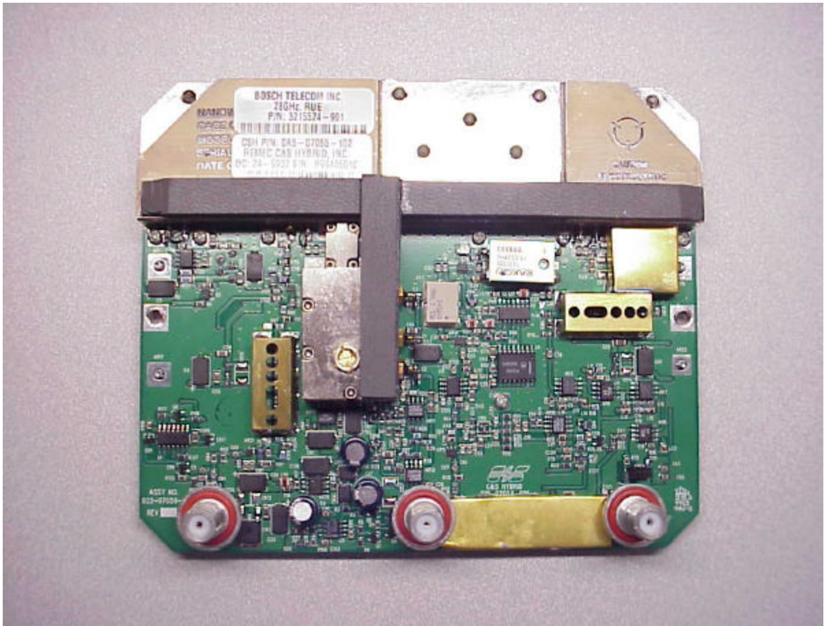
Figure 9-1 Roof Unit Electronics Board
