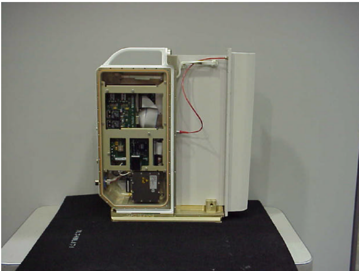
Figure 9-1 Node Transmitter side view cover removed
