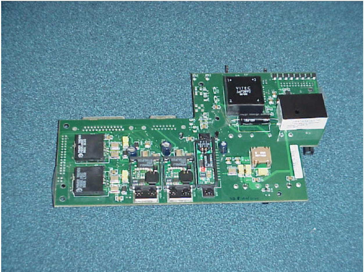
Figure 9-5 Node Transmitter Digital Board - Backside
