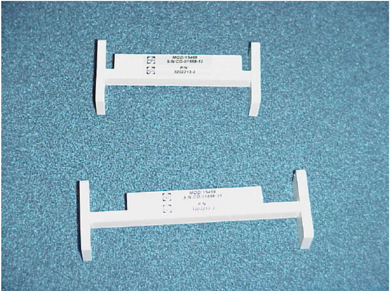
Figure 9-6 Node Transmitter Waveguide Filter
