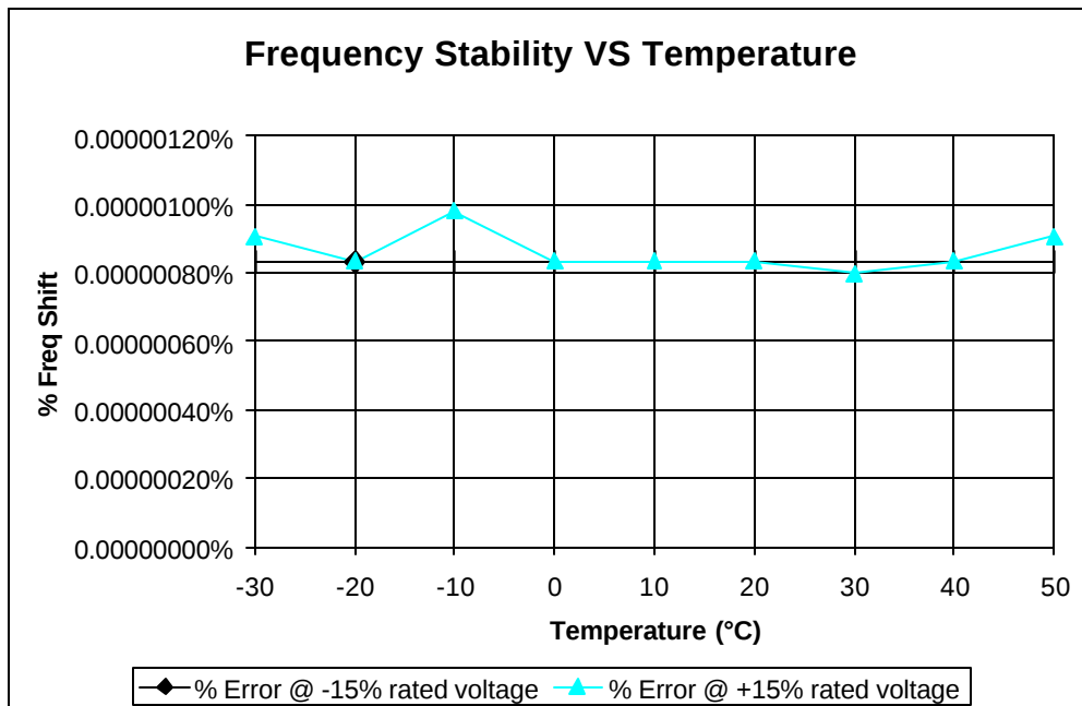
Figure E – 1 Frequency Stability Graph, SpectraPoint High Gain Node Transmitter
