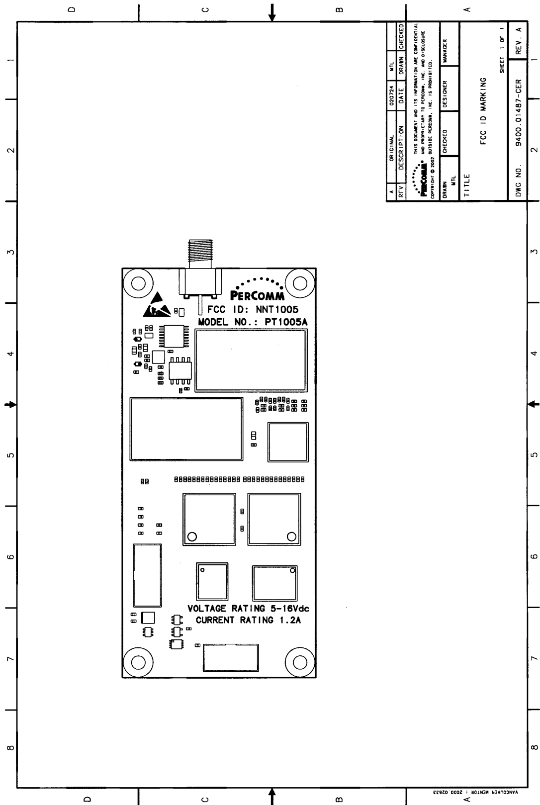
FCC ID Marking is done in silkscreen on the topside of the PCB.
