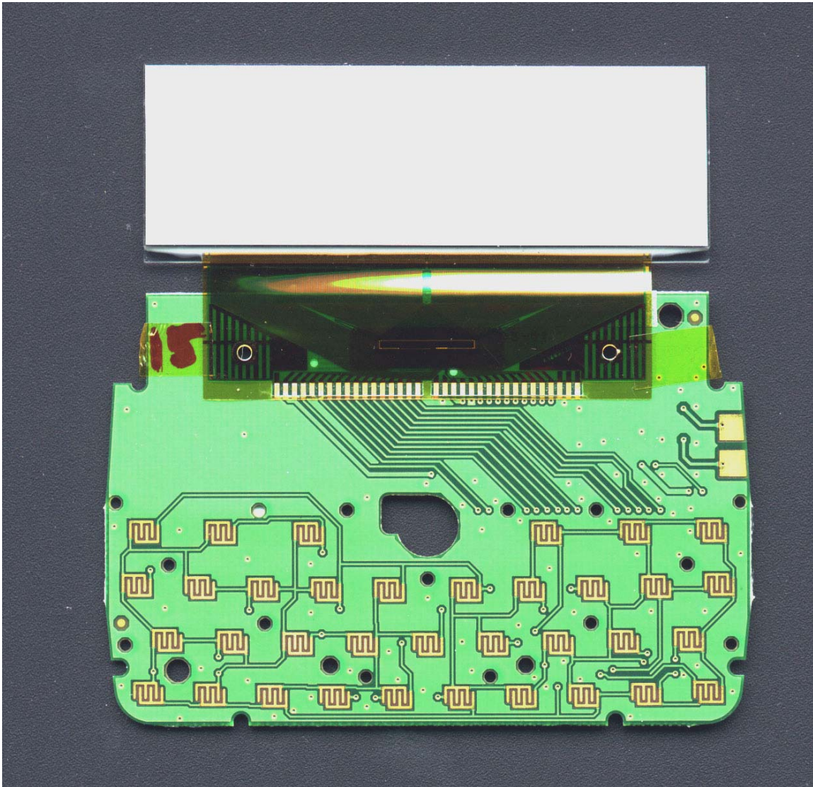
Top view of the display board of the e80 device
