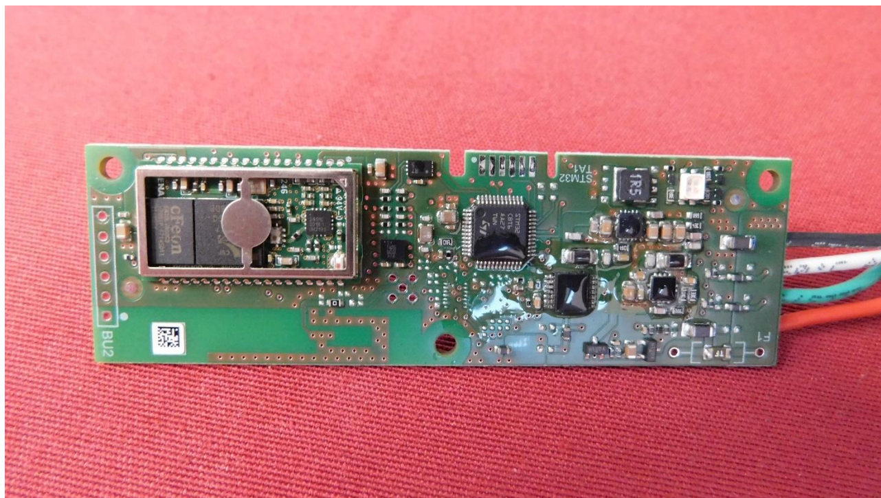
Picture 7: PCB of final product (not tested) – top side – without shielding
