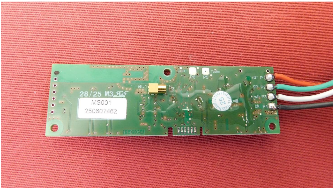
Picture 5: PCB of the EUT – bottom side – with temporary antenna port
