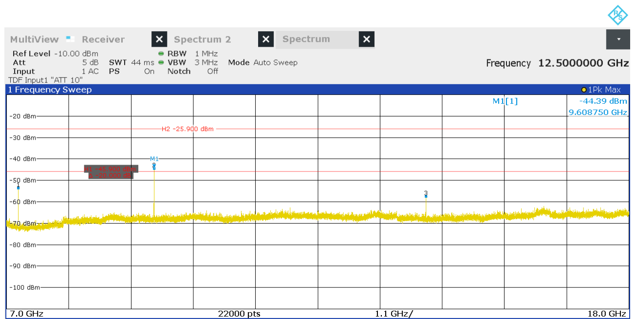
Figure 25: Chart of emissions test from 7 GHz to 18 GHz on lowest channel, Pk
