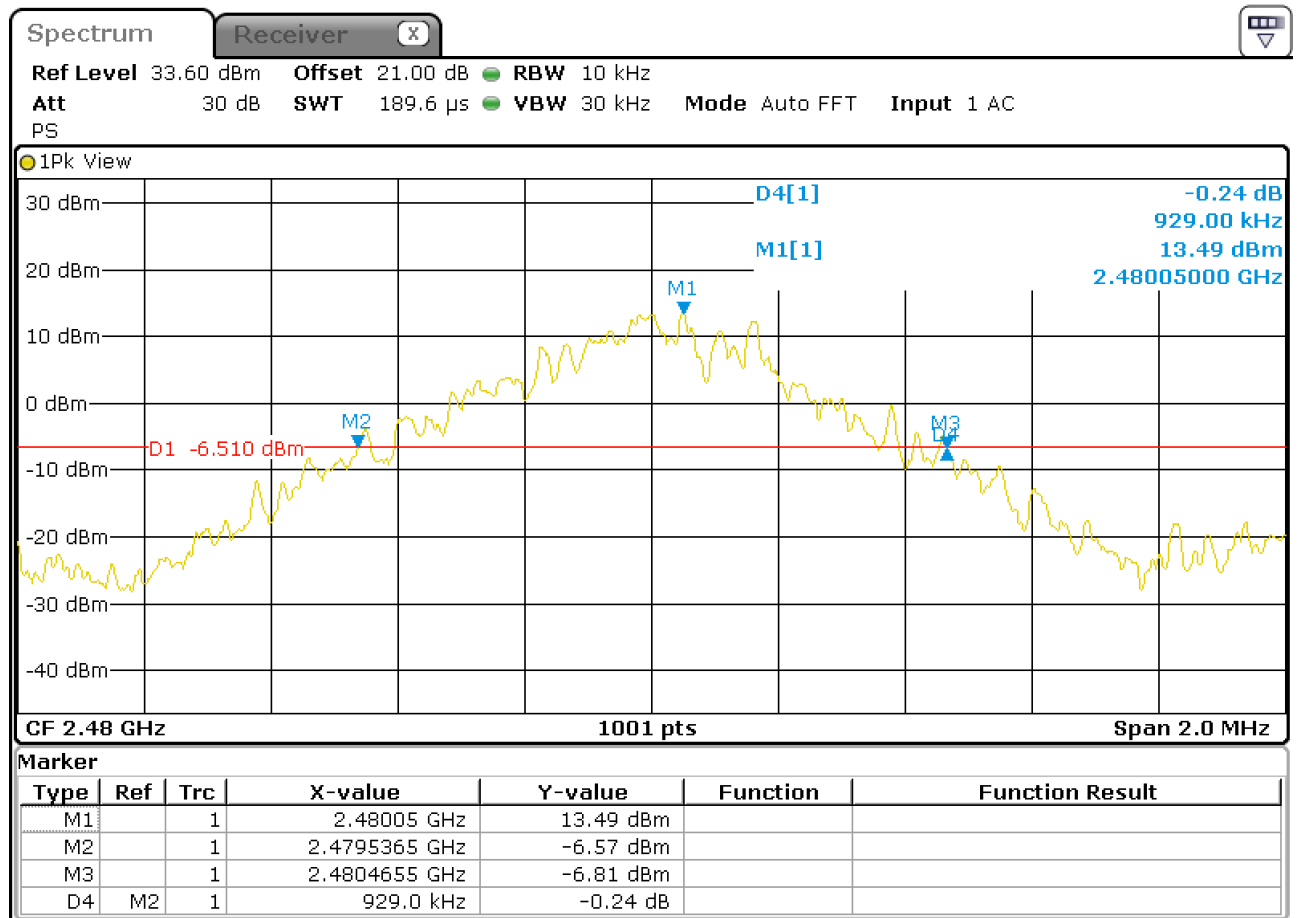
Figure 8: Chart of 20 dB bandwidth test on highest channel
