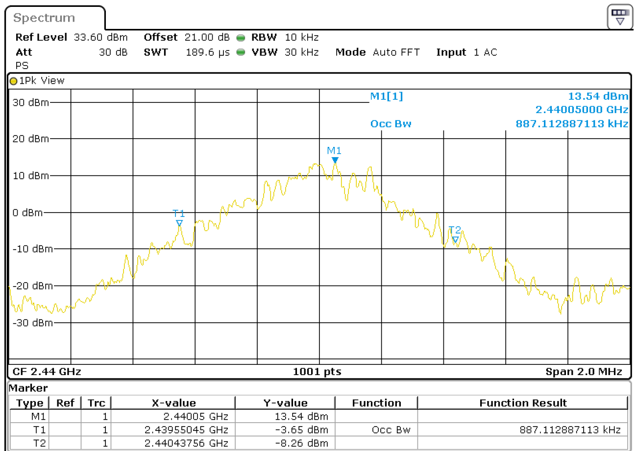
Figure 10: Chart of occupied bandwidth test on middle channel
