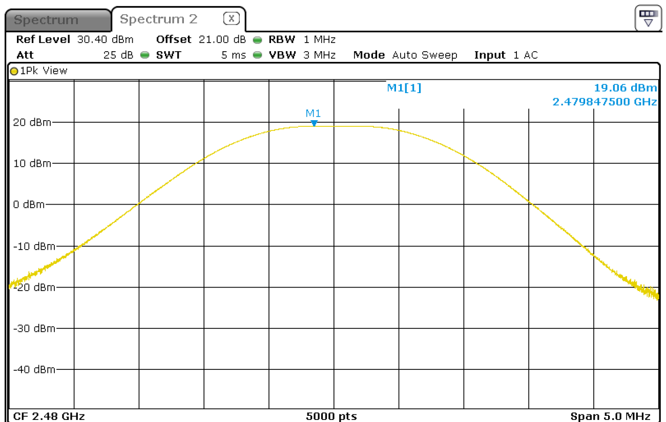
Figure 15: Chart of conducted output power on highest channel
