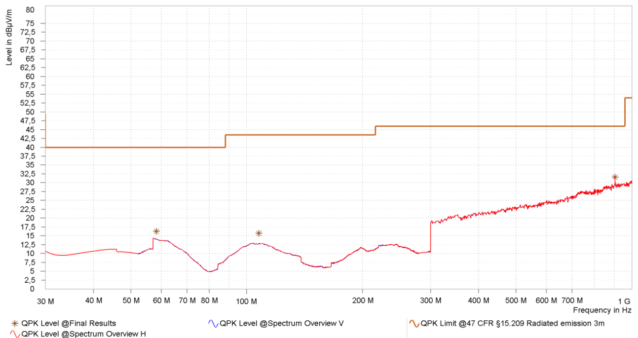
Figure 36: Chart of radiated emissions test from 30 MHz to 1 GHz on middle channel, EUT position X, antenna polarization horizontal and vertical
