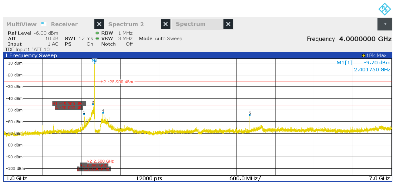
Figure 24: Chart of emissions test from 1 GHz to 7 GHz on lowest channel, Pk
