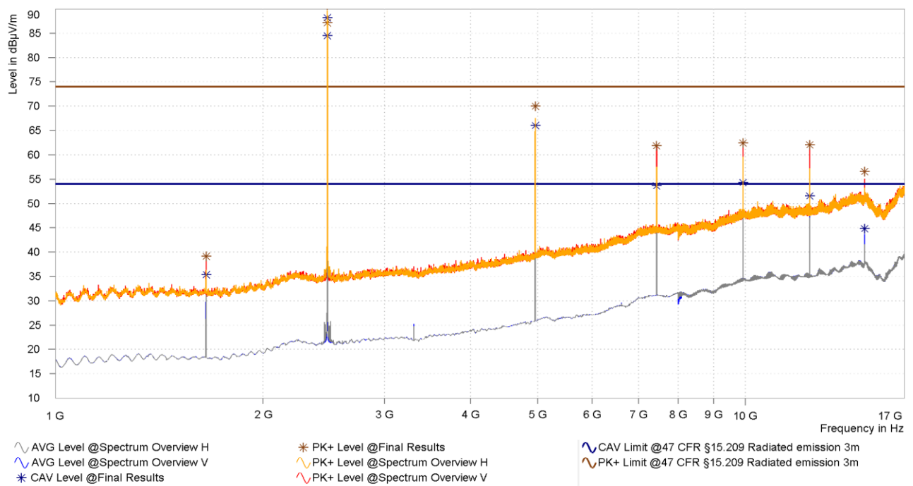
Figure 41: Chart of radiated emissions pre-measurement from 1 GHz to 17 GHz on highest channel, EUT position X, antenna polarization horizontal and vertical
