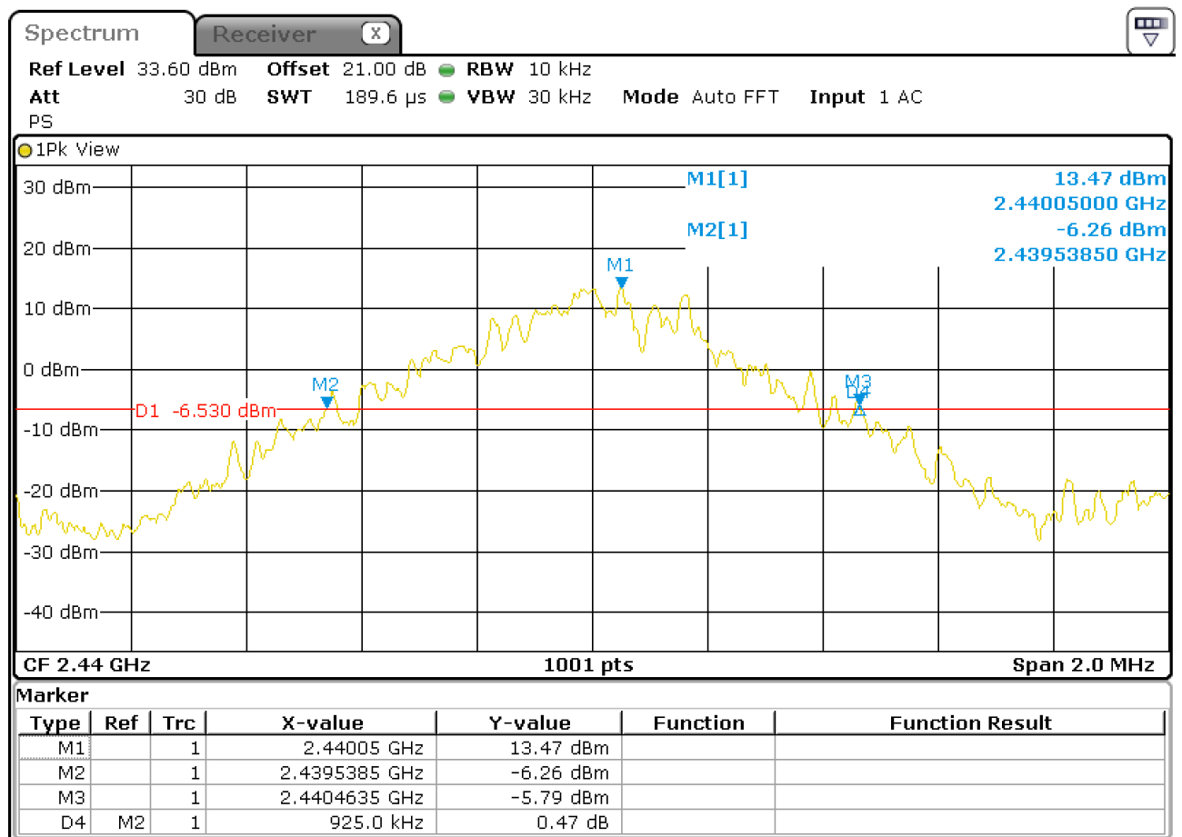
Figure 7: Chart of 20 dB bandwidth test on middle channel
