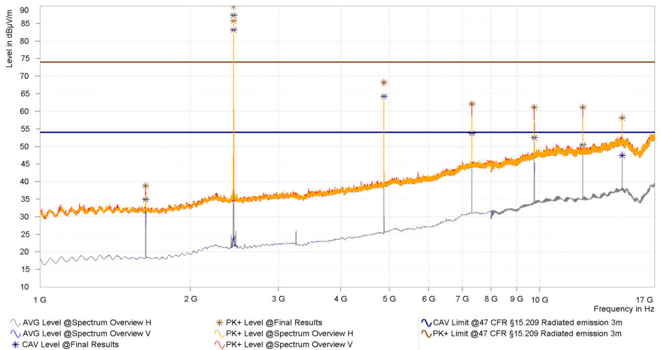
Figure 39: Chart of radiated emissions pre-measurement from 1 GHz to 17 GHz on middle channel, EUT position X, antenna polarization horizontal and vertical
