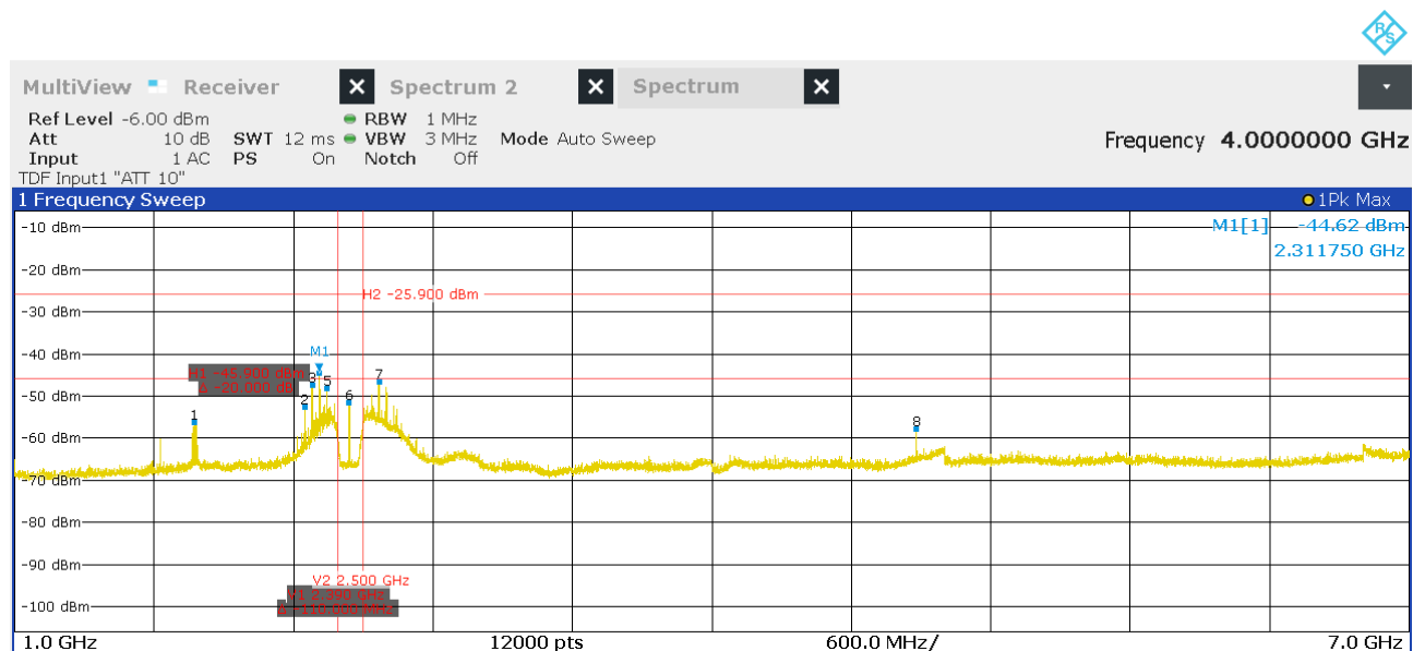
Figure 28: Chart of emissions test from 1 GHz to 7 GHz on middle channel, Pk
