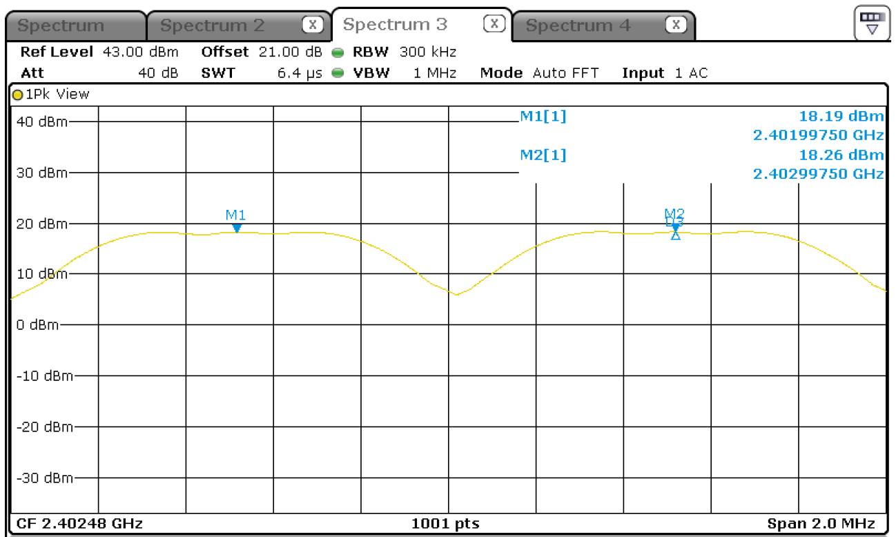
Figure 16: Chart of carrier frequency separation_channels 01and 02
