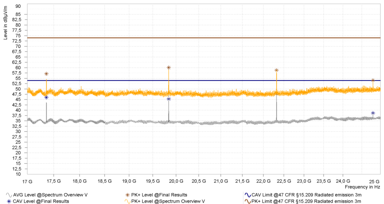
Figure 42: Chart of emissions measurement from 17 GHz to 25 GHz on highest channel, EUT position X, antenna polarization vertical
