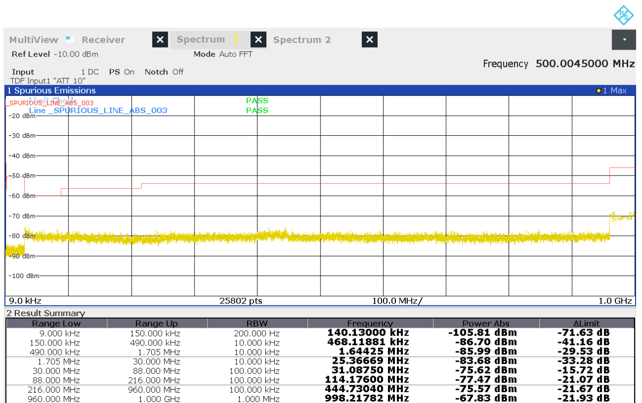
Figure 31: Chart of emissions test from 9 kHz to 1 GHz on highest channel, Pk
