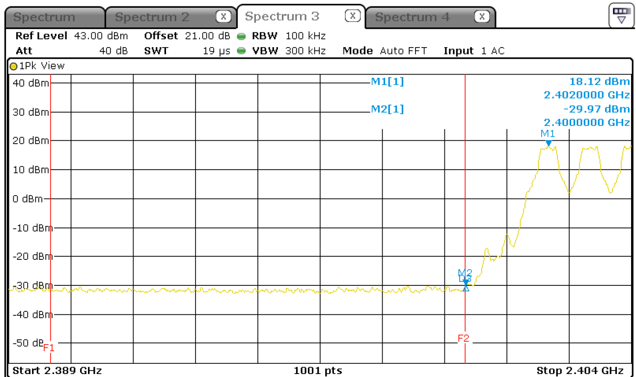
Figure 21: Chart of lower band-edge measurement in hopping mode
