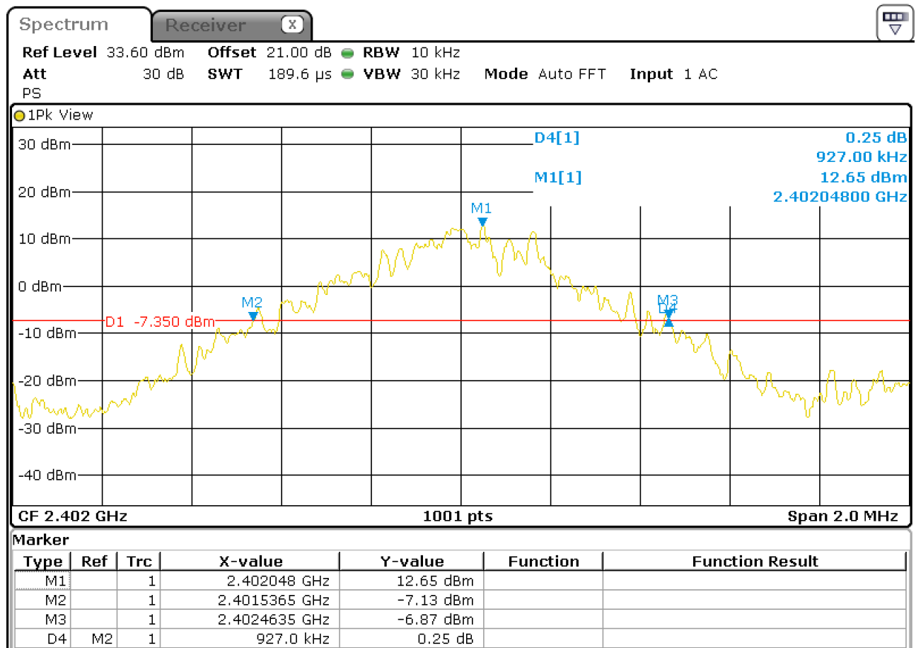
Figure 6: Chart of 20 dB bandwidth test on lowest channel
