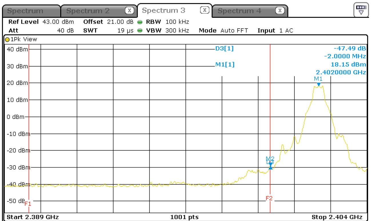
Figure 20: Chart of lower band-edge measurement in non-hopping mode on lowest channel
