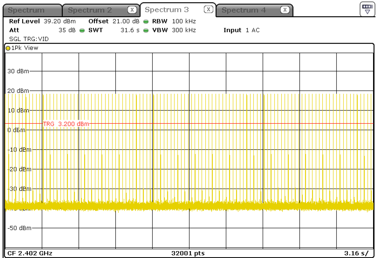
Figure 19: Number of transmission bursts within a 31.6 second period on lowest channel
