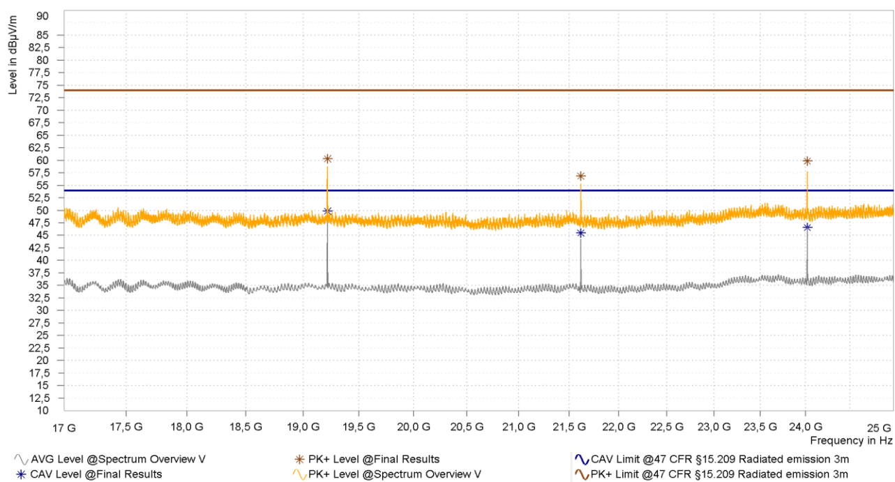
Figure 38: Chart of radiated emissions measurement from 17 GHz to 25 GHz on lowest channel, EUT position X, antenna polarization vertical
