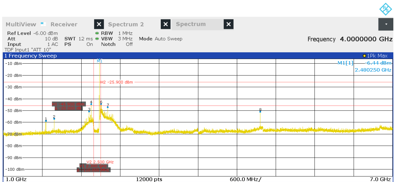
Figure 32: Chart of emissions test from 1 GHz to 7 GHz on highest channel, Pk
