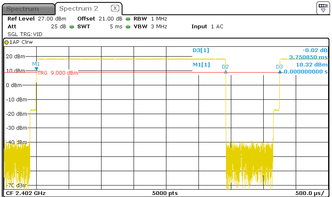
Figure 12: Chart of the duty cycle measurement of 1 transmission interval on the lowest channel
