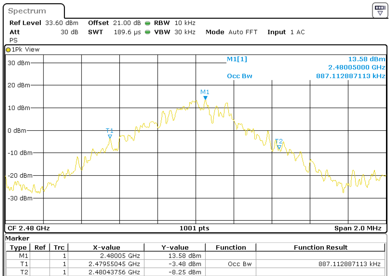
Figure 11: Chart of occupied bandwidth test on highest channel
