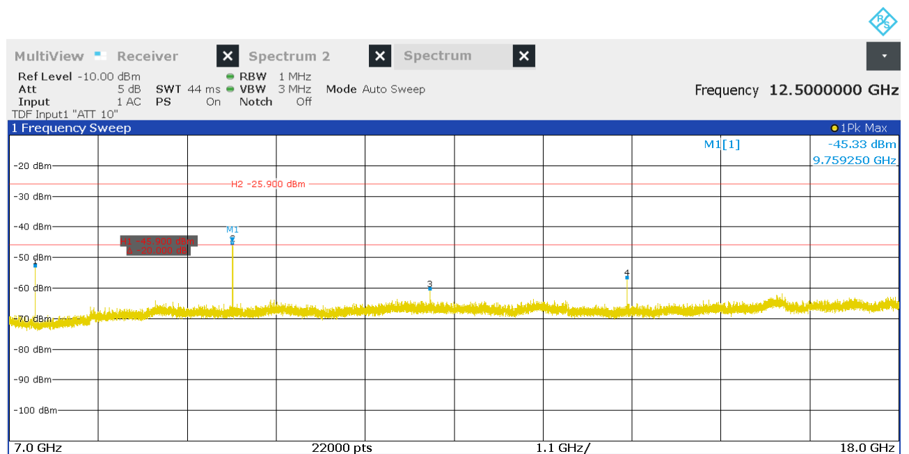
Figure 29: Chart of emissions test from 7 GHz to 18 GHz on middle channel, Pk
