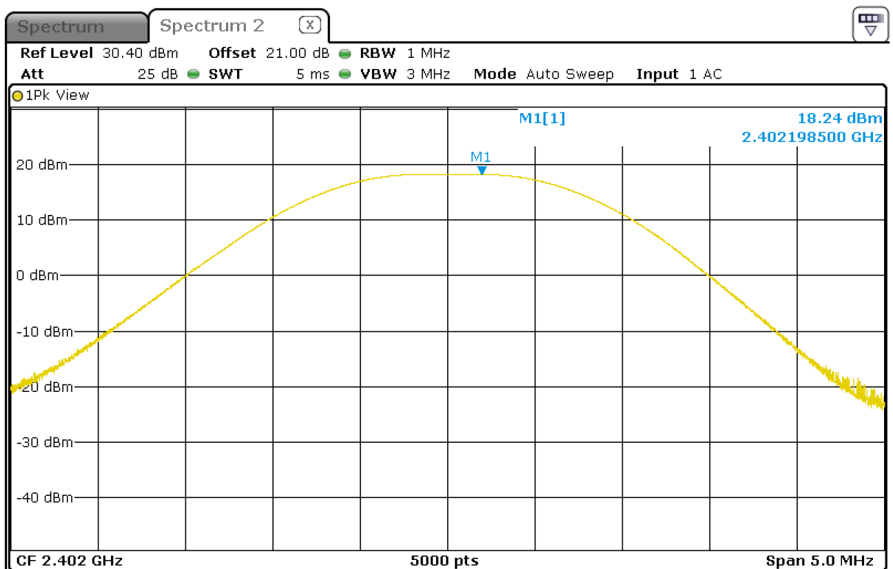
Figure 13: Chart of conducted output power on lowest channel
