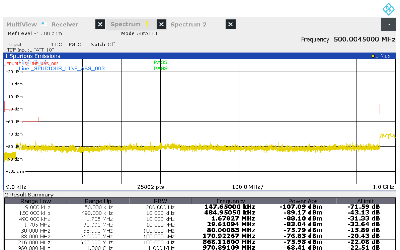
Figure 27: Chart of emissions test from 9 kHz to 1 GHz on middle channel, Pk
