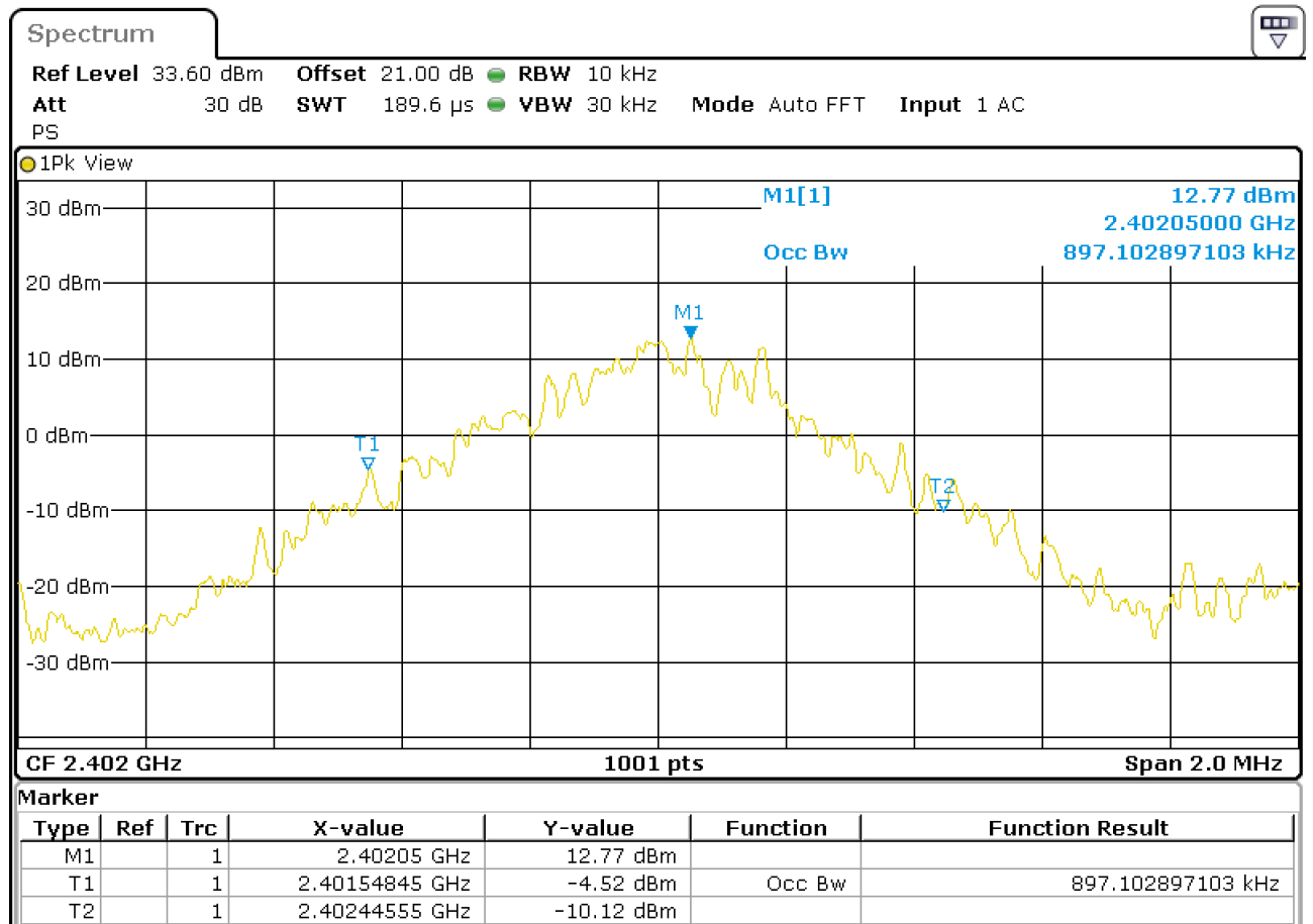
Figure 9: Chart of occupied bandwidth test on lowest channel
