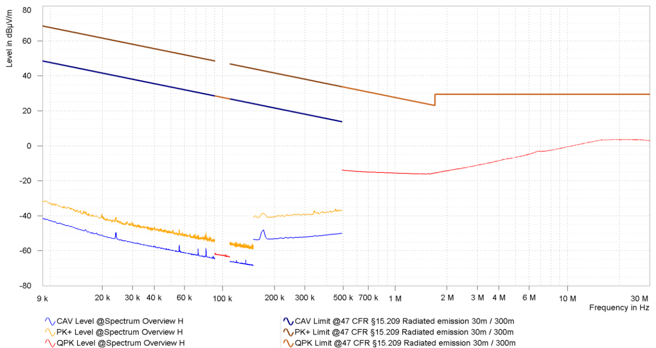
Figure 35: Chart of emissions test below 30 MHz on middle channel, EUT position X, antenna parallel
