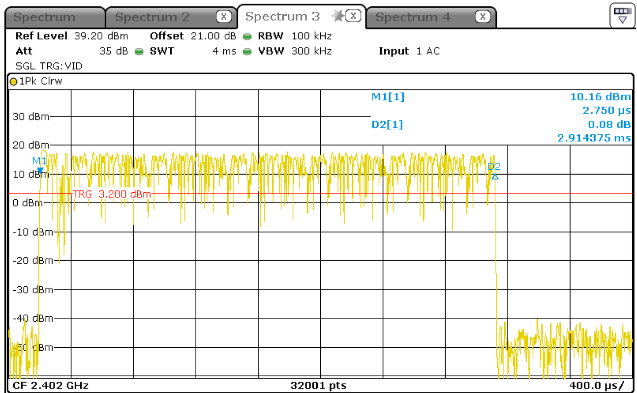
Figure 18: Length of 1 transmission burst on lowest channel
