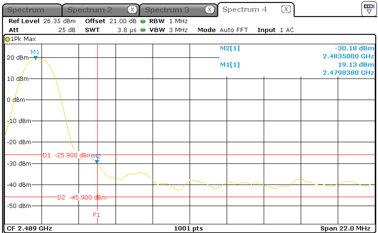
Figure 22: Chart of upper band-edge measurement in non-hopping mode on highest channel (PK)
