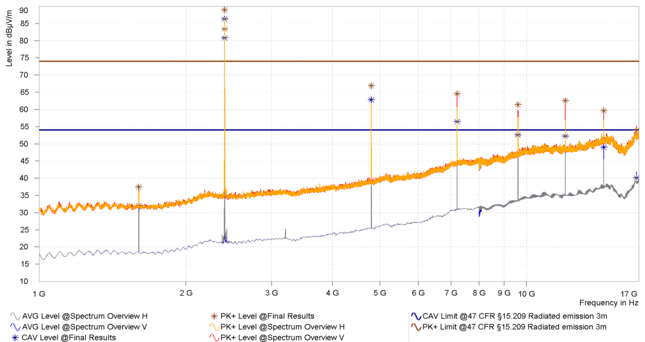
Figure 37: Chart of radiated emissions pre-measurement from 1 GHz to 17 GHz on lowest channel, EUT position X, antenna polarization horizontal and vertical
