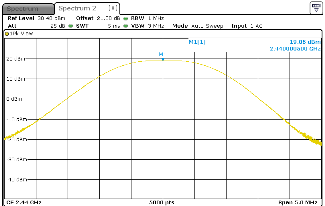
Figure 14: Chart of conducted output power on middle channel
