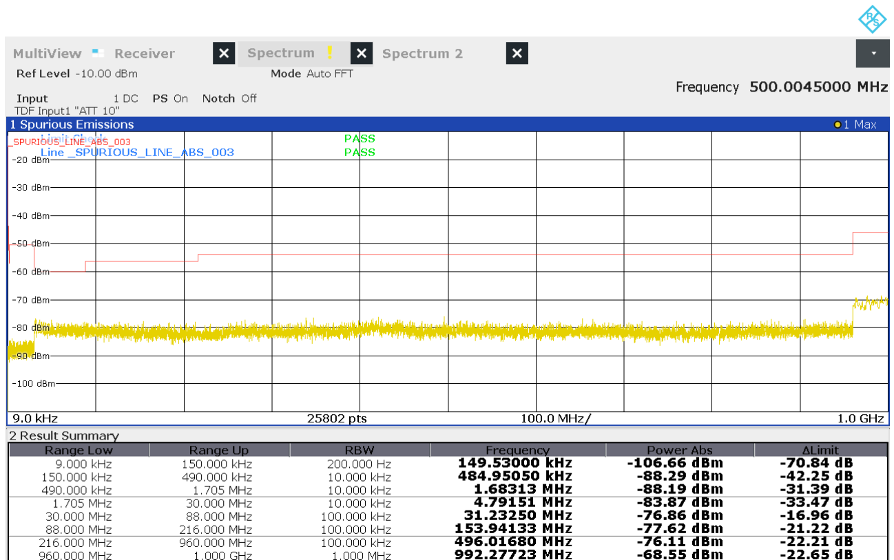
Figure 23: Chart of emissions test from 9 kHz to 1 GHz on lowest channel, Pk
