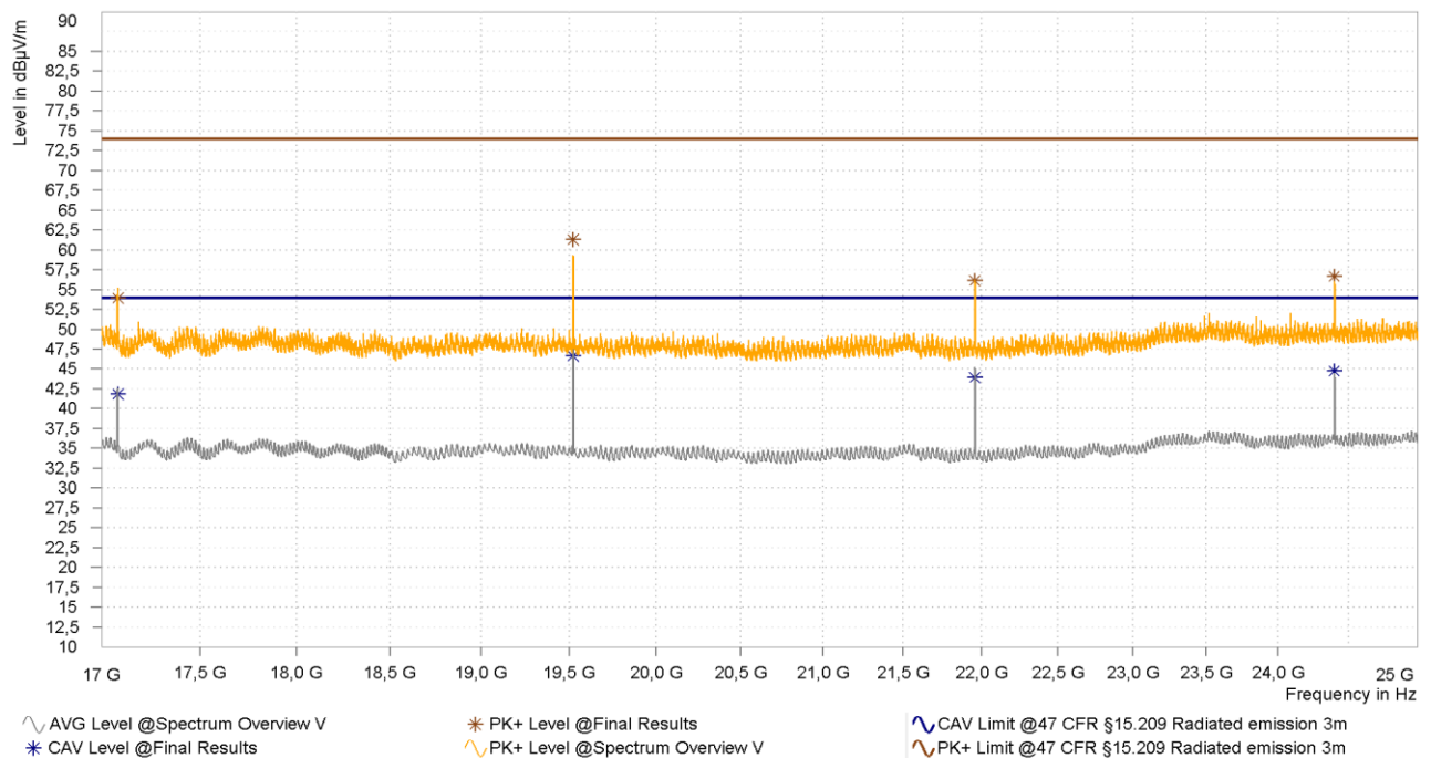
Figure 40: Chart of emissions measurement from 17 GHz to 25 GHz on middle channel, EUT position X, antenna polarization vertical
