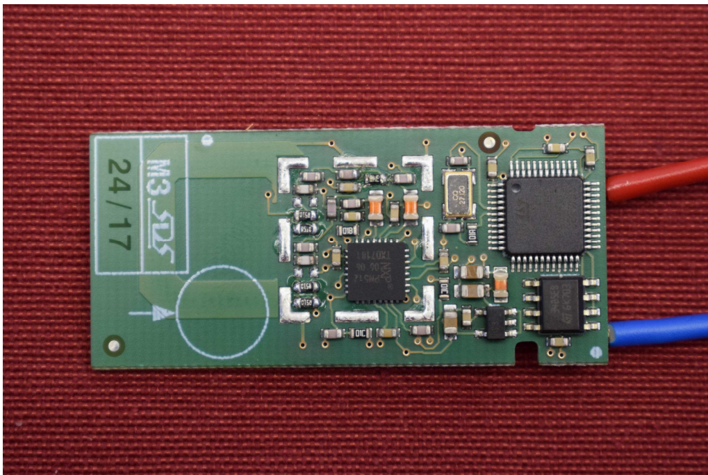
Picture 2: EUT – top side, without shielding
