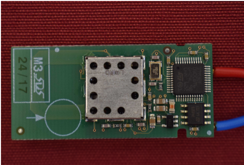
Picture 1: EUT - top side, with shielding
