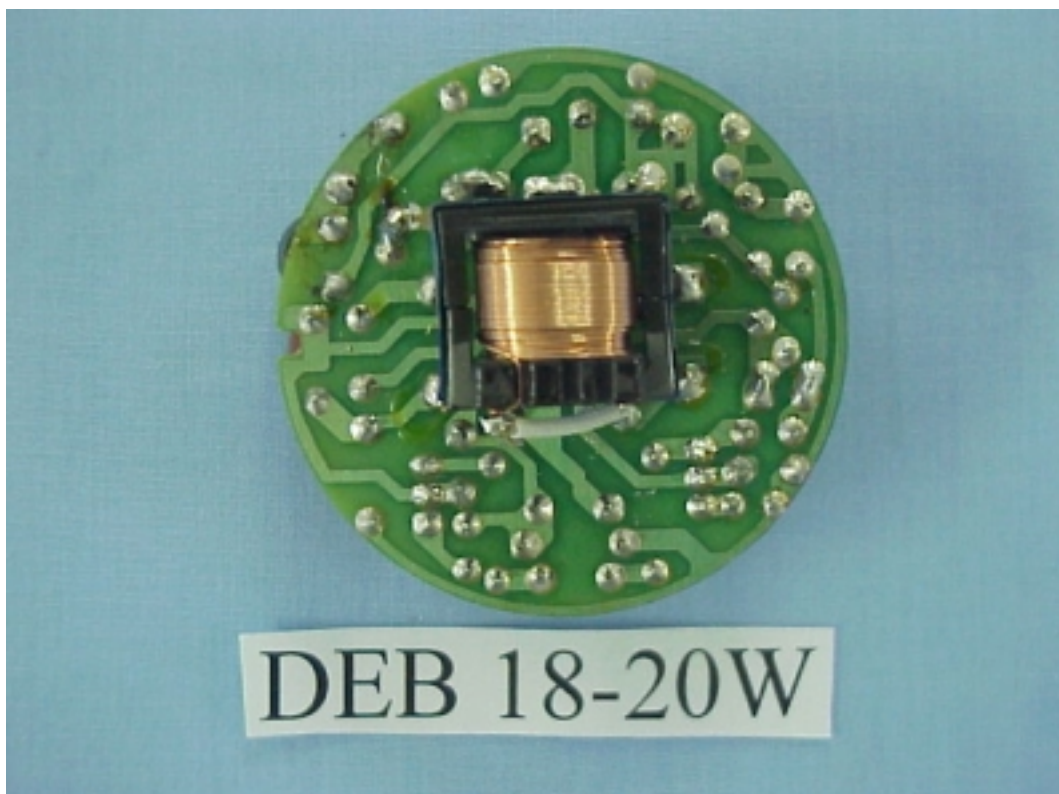
FIGURE 7 ELECTRONIC ENERGY SAVING LAMP (M/N: DEB/18~20W) MAIN BOARD (SOLDERED SIDE)
