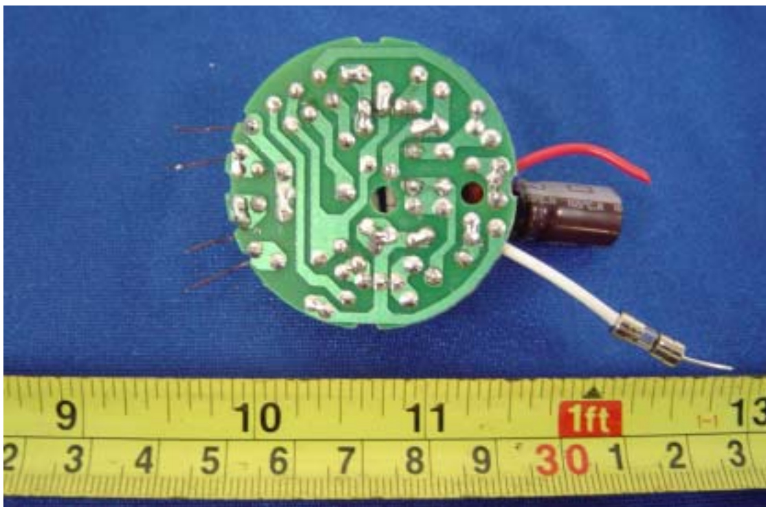
DEF20W _Internal Photos For Solder View
