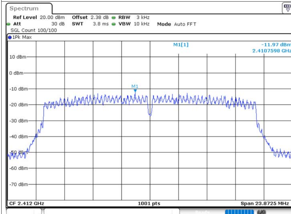
PSD NVNT n20 2412MHz Ant1
