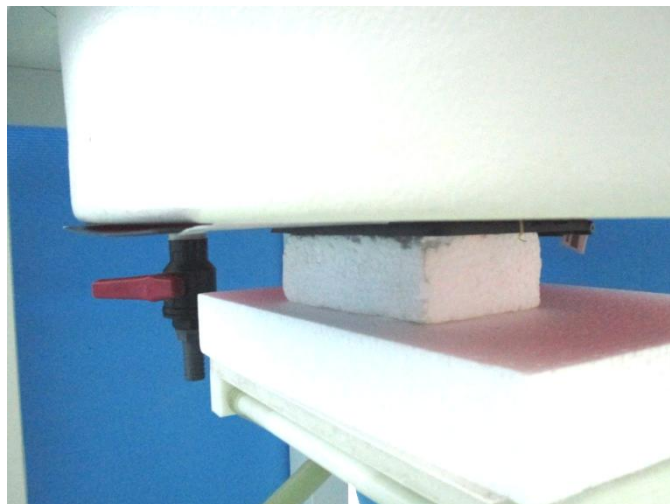
Fig-4.2 Rear Face of EUT with 0 cm Gap (EUT + Holster 2)
