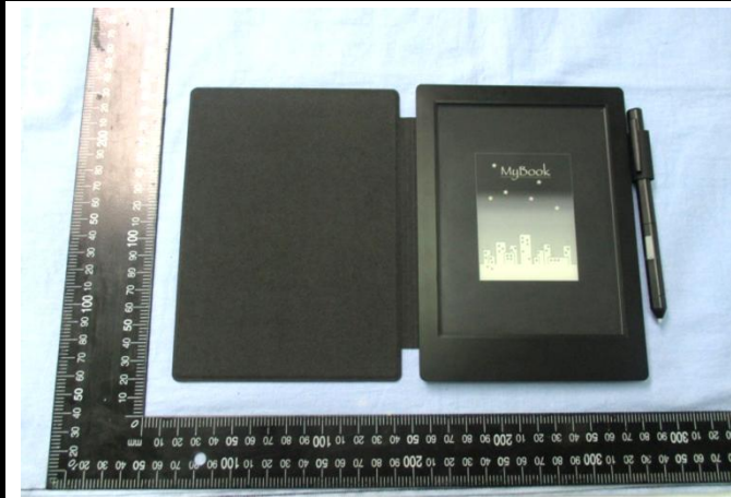
EUT with Holster 1
