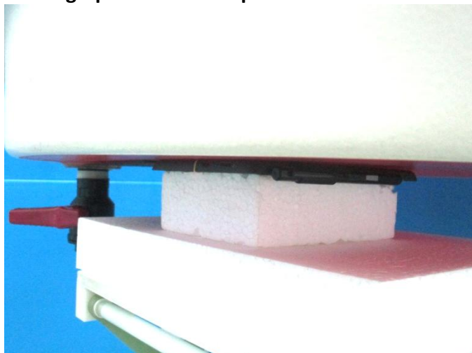
Fig-4.1 Rear Face of EUT with 0 cm Gap (EUT + Holster 1)
