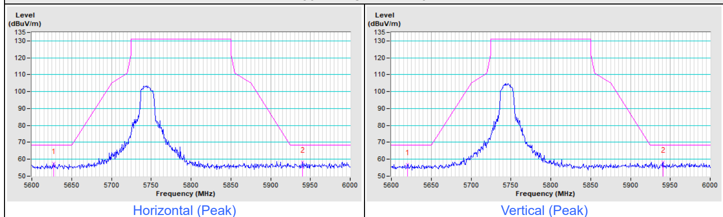
802.11a Channel 149
