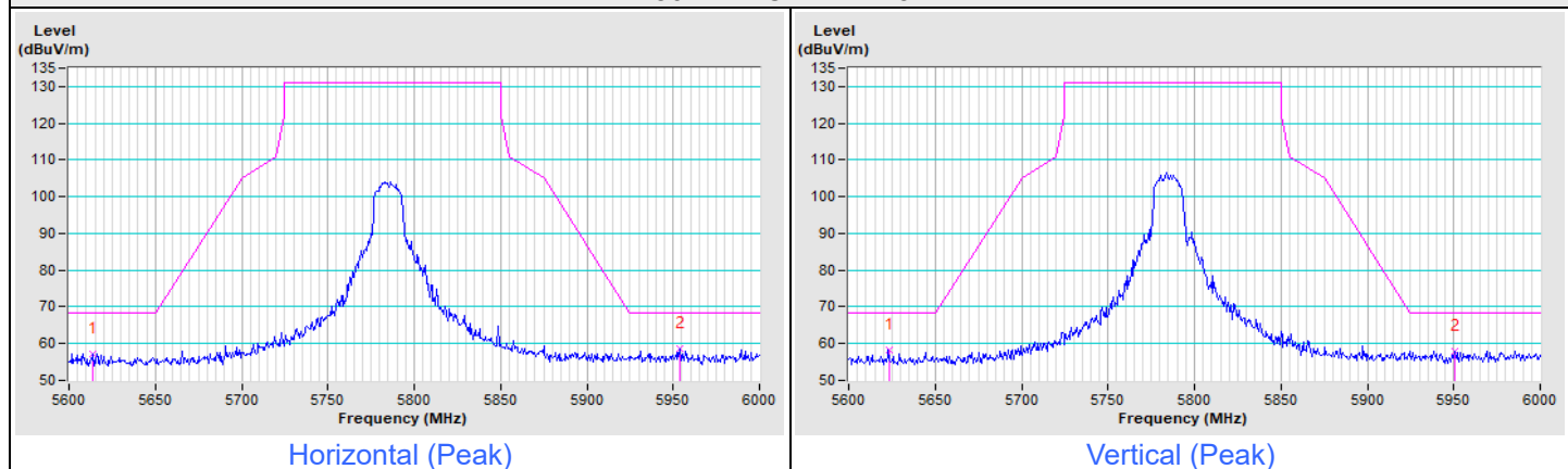
802.11a Channel 157
