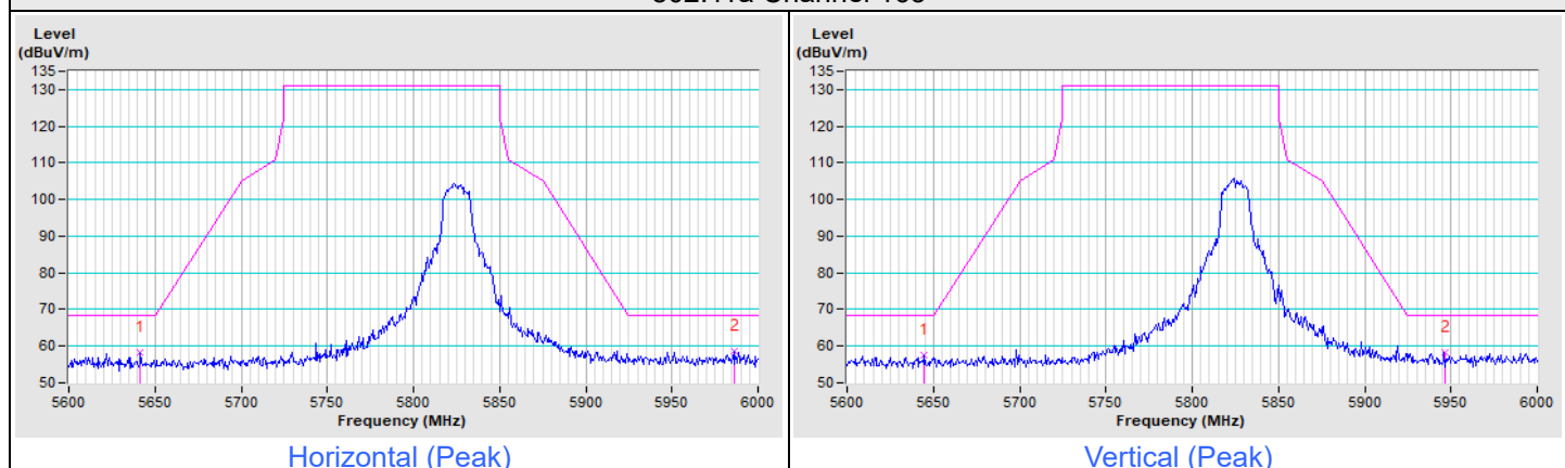
802.11a Channel 165
