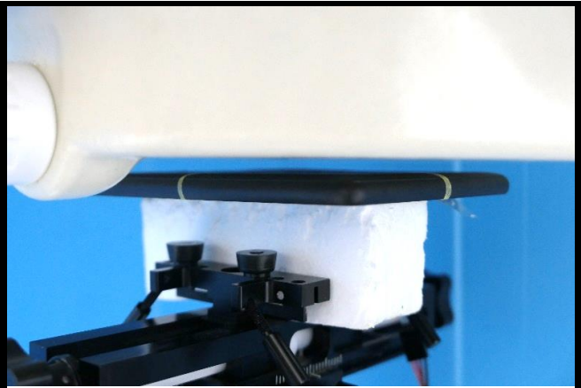
Rear Face of EUT Mode Tested at 5 mm
