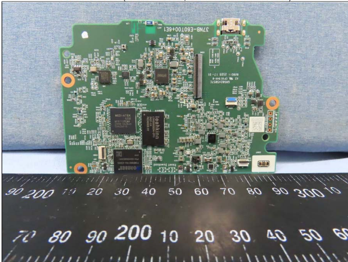
PCB with eMMC (Brand: FORESEE, Model: FEMDNN016G-A3A55) and DRAM LP-DDR4 (Brand: Leahkinn, Model: LTHS0005GS4-ZPI1)
