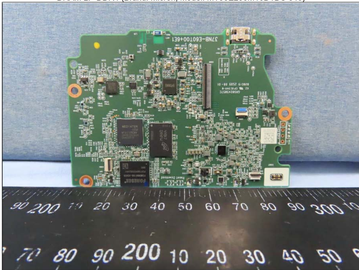
PCB with eMMC (Brand: FORESEE, Model: FEMDNN016G-A3A55) and DRAM LP-DDR4 (Brand: Micron, Model: MT53E256M16D1DS-046)
