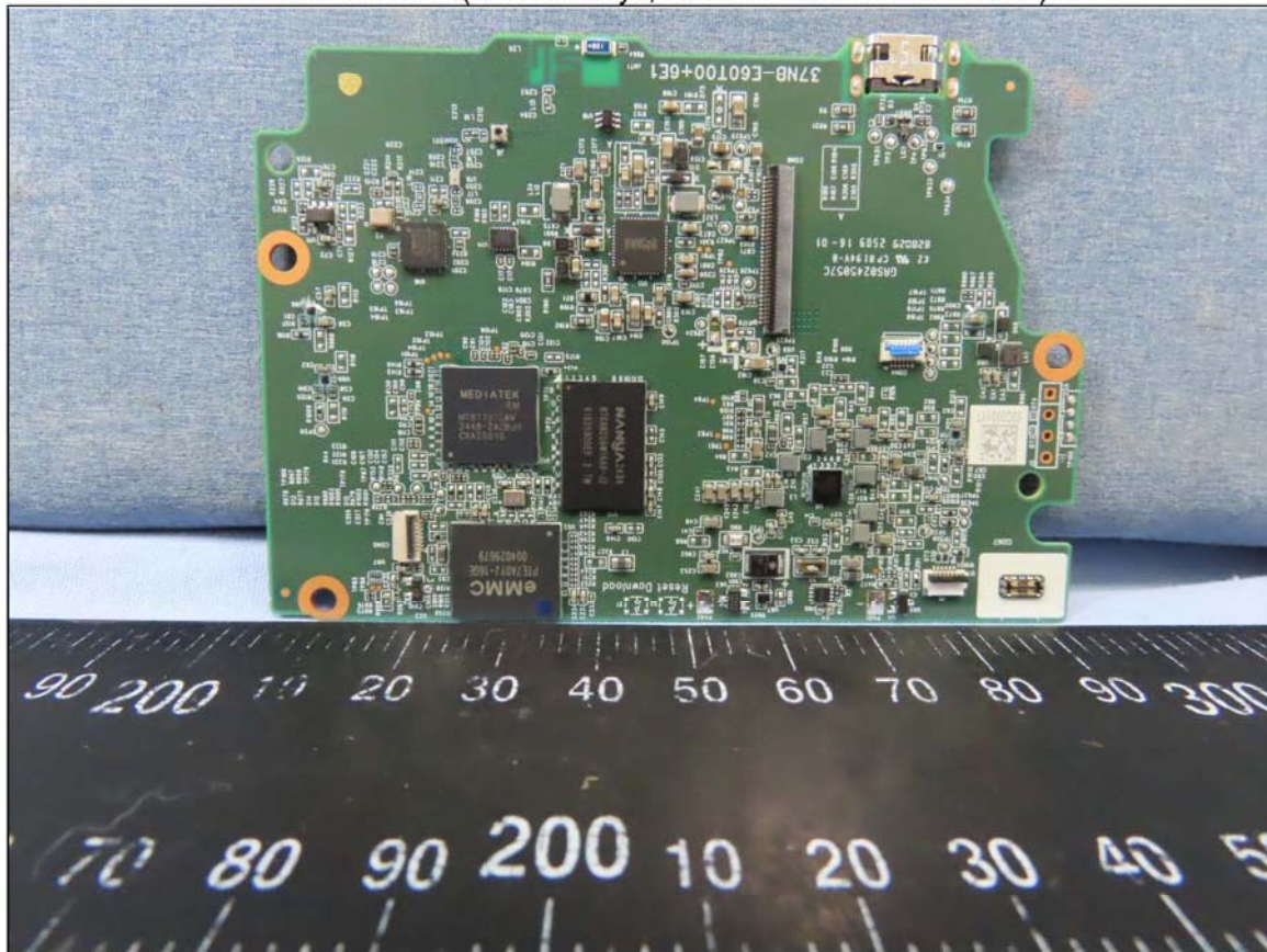
PCB with eMMC (Brand: Phison, Model: PTE7A0YJ-16GE) and DRAM LP-DDR4 (Brand: Nanya, Model: NT6AN256M16AV-J2)
