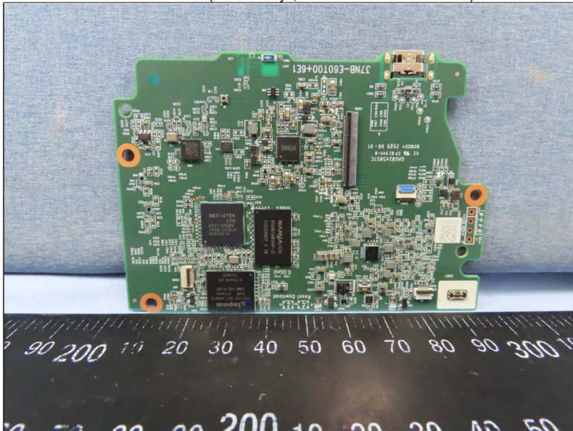
PCB with eMMC (Brand: Kingston, Model: EMMC16G-PJ30-GA02) and DRAM LP-DDR4 (Brand: Nanya, Model: NT6AN256M16AV-J2)
