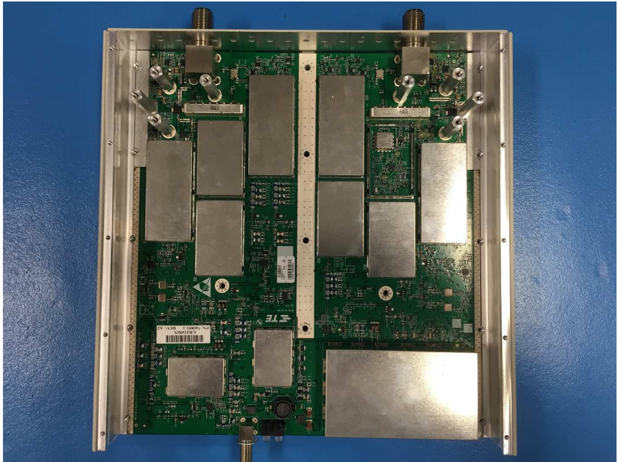
Top Side in Chassis
