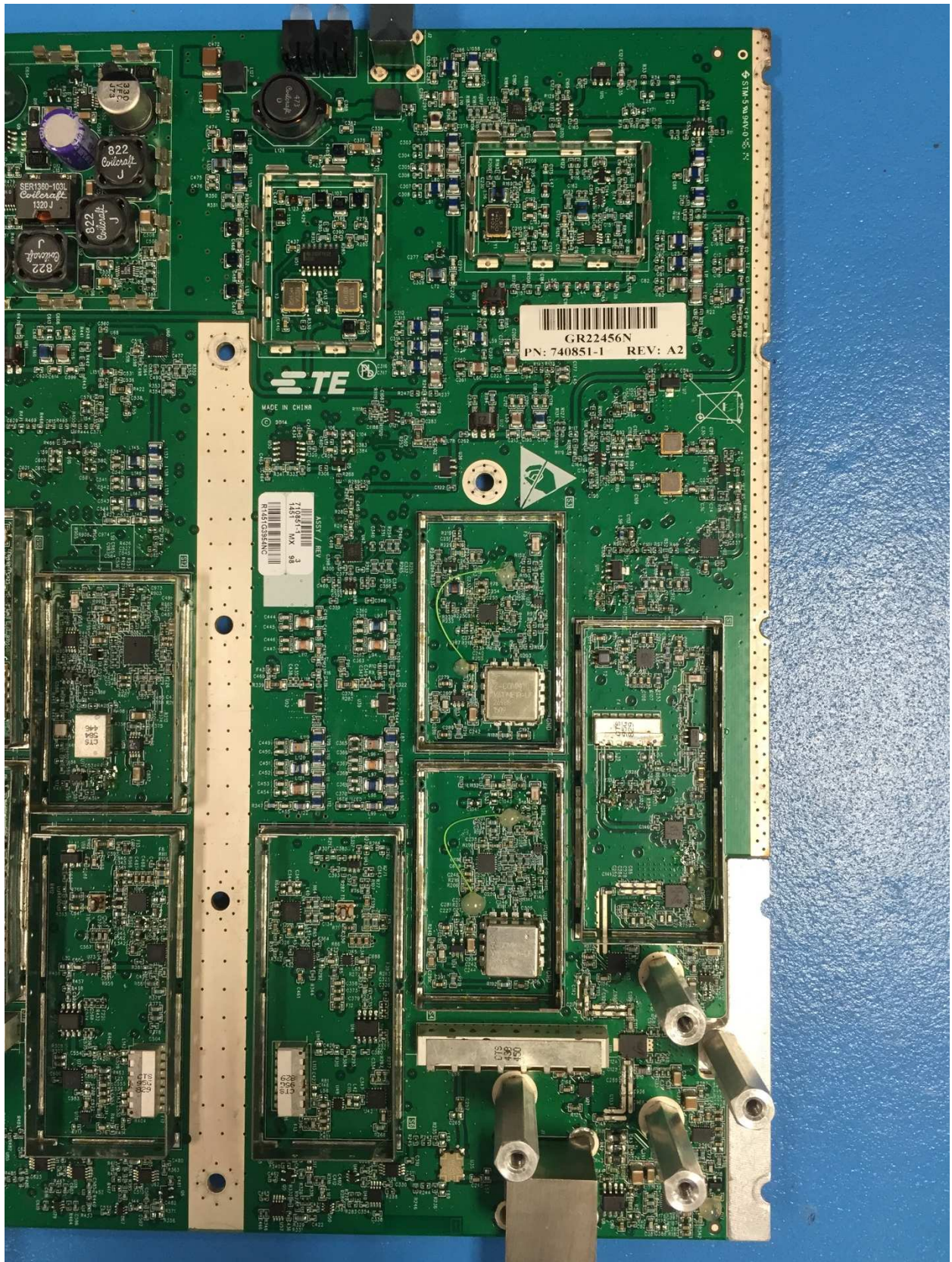
Top Right Side
