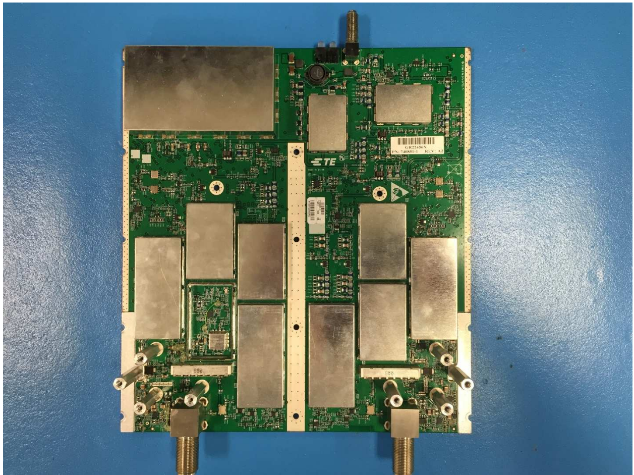
Top Side (Shielded)
