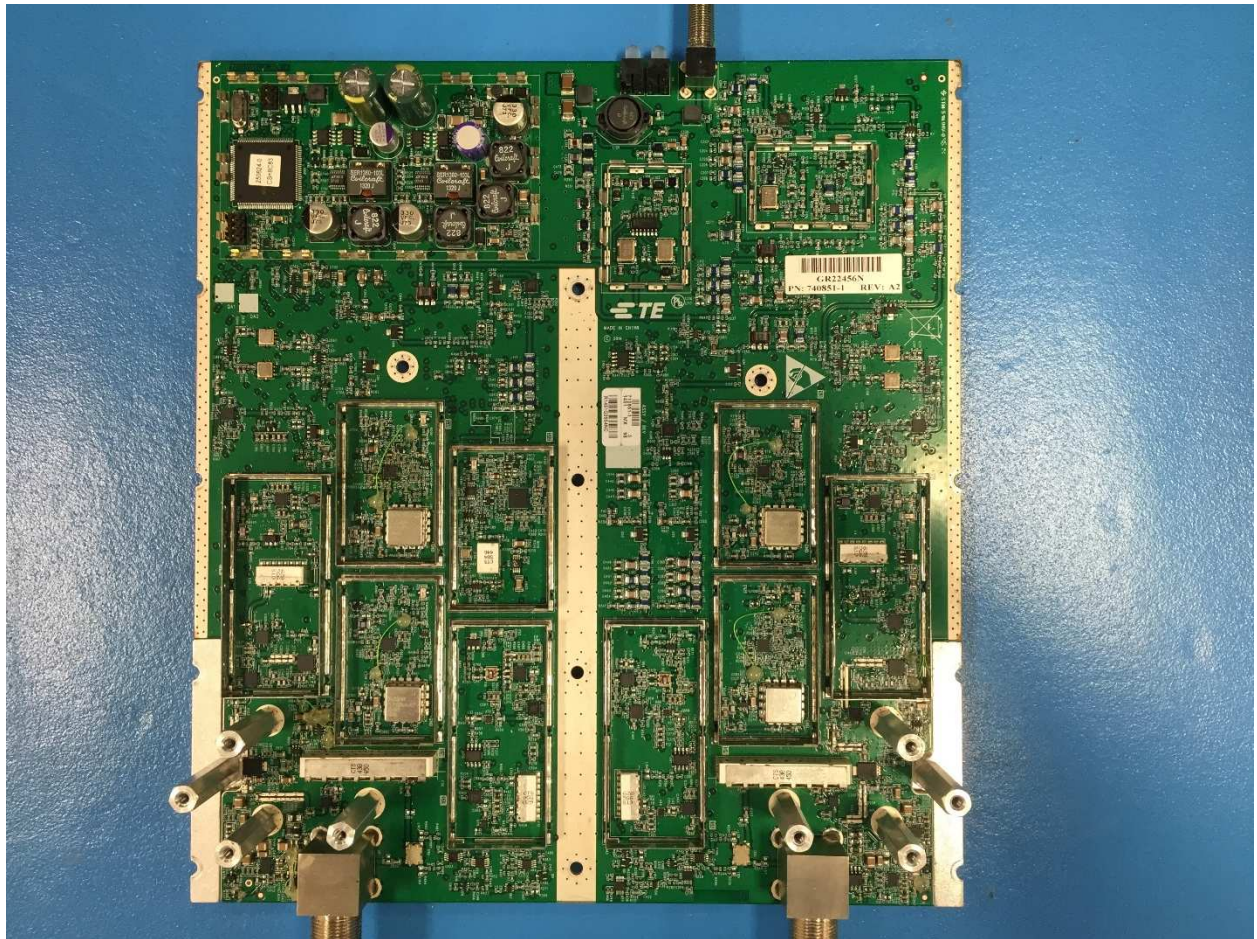
Top Sided (unshielded)
