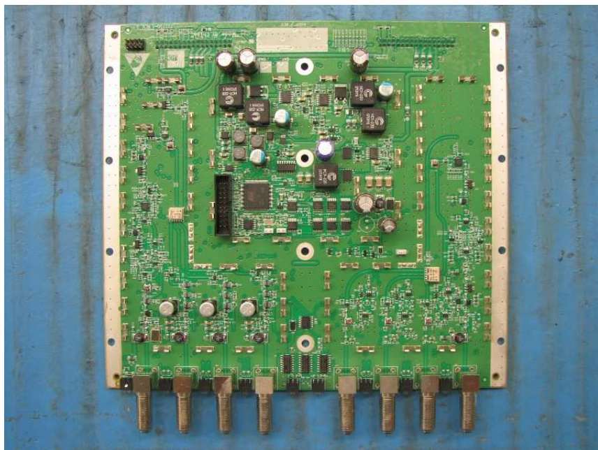
PCB IF Assembly Bottom View without shielding- MRAU
