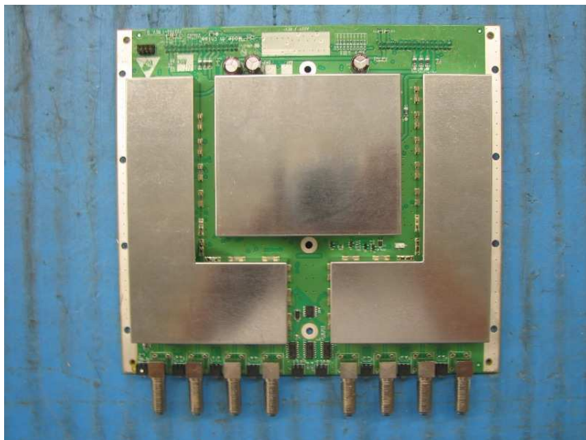
PCB IF Assembly Bottom View with shielding- MRAU
