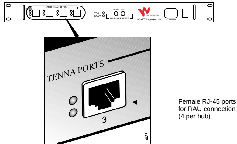
Figure 4-4 RJ-45 Ports on the Expansion Hub
