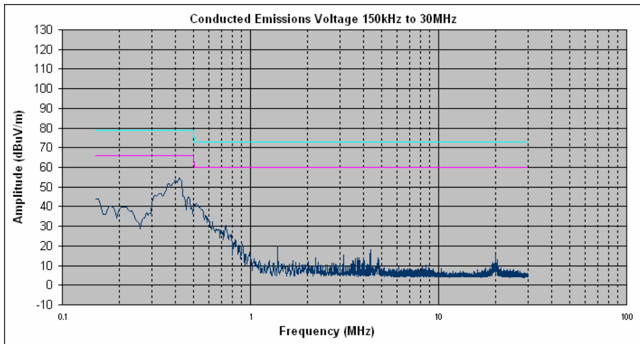
Conducted Emission, Phase Line Plots, Top Unit
