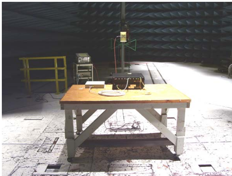
Photograph 7. Radiated Emission Limits Test Setup, 1 GHz to 10 GHz, Back View
