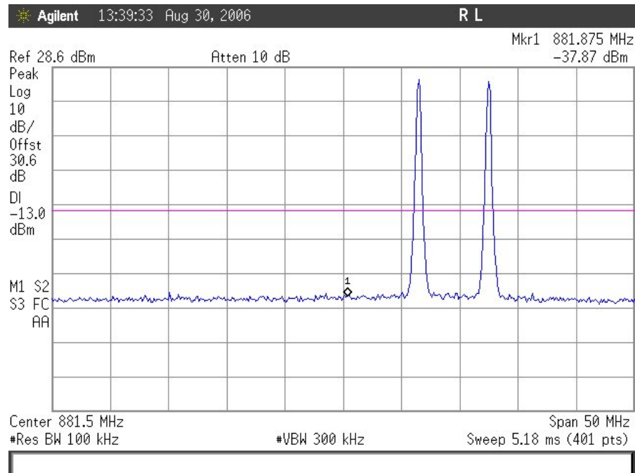
AMPS Downlink Intermodulation, High End - Cellular
