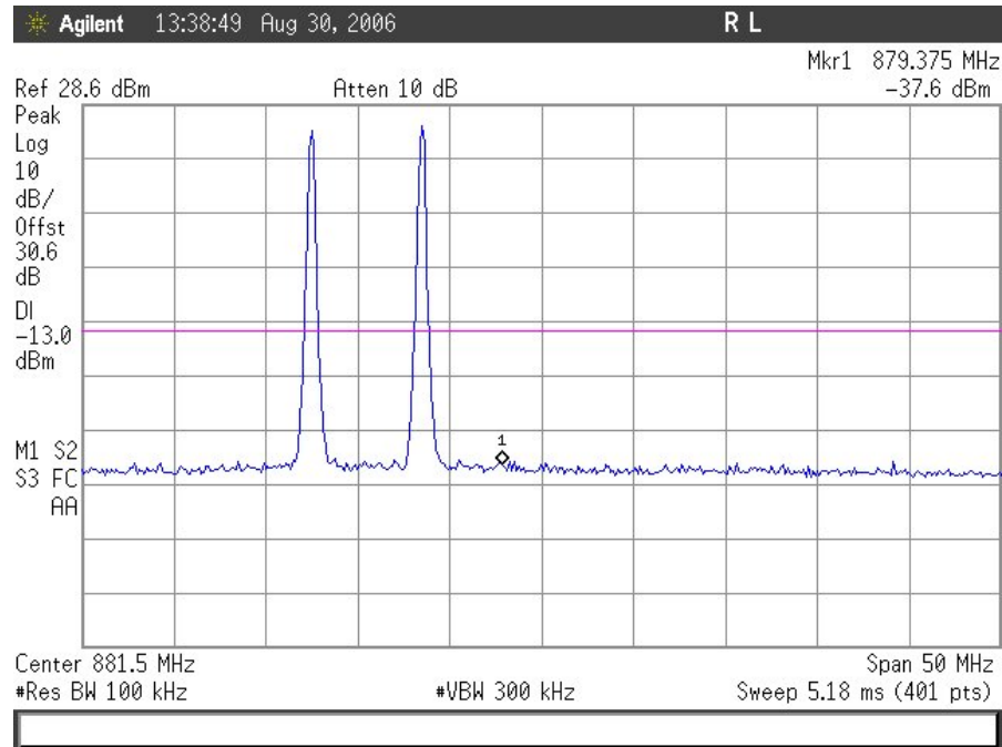
AMPS Downlink Intermodulation, Low End - Cellular
