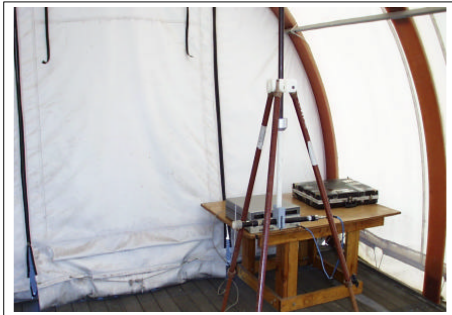
SUBSTITUTION MEASUREMENTS (800MHz)
