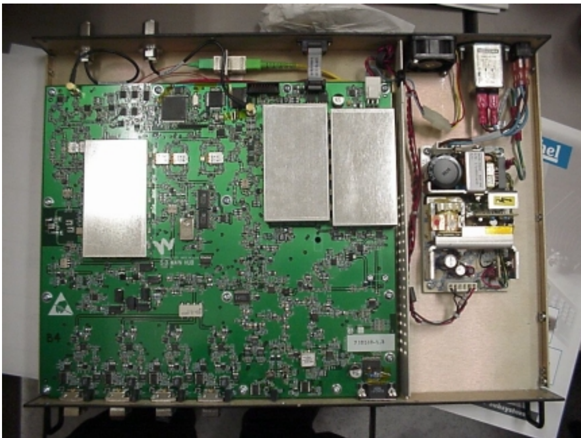
Inside Main hub (with shields)
