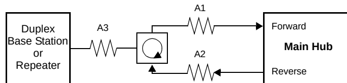
Figure 6-3 Main Hub to Duplex Base Station or Repeater Connections
