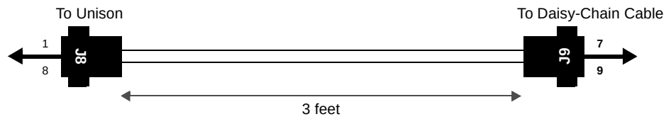
Figure 7-11 Alarm Sense Adapter Cable
