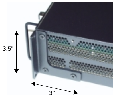
Right Rack Mounting Bracket as installed from the factory.
