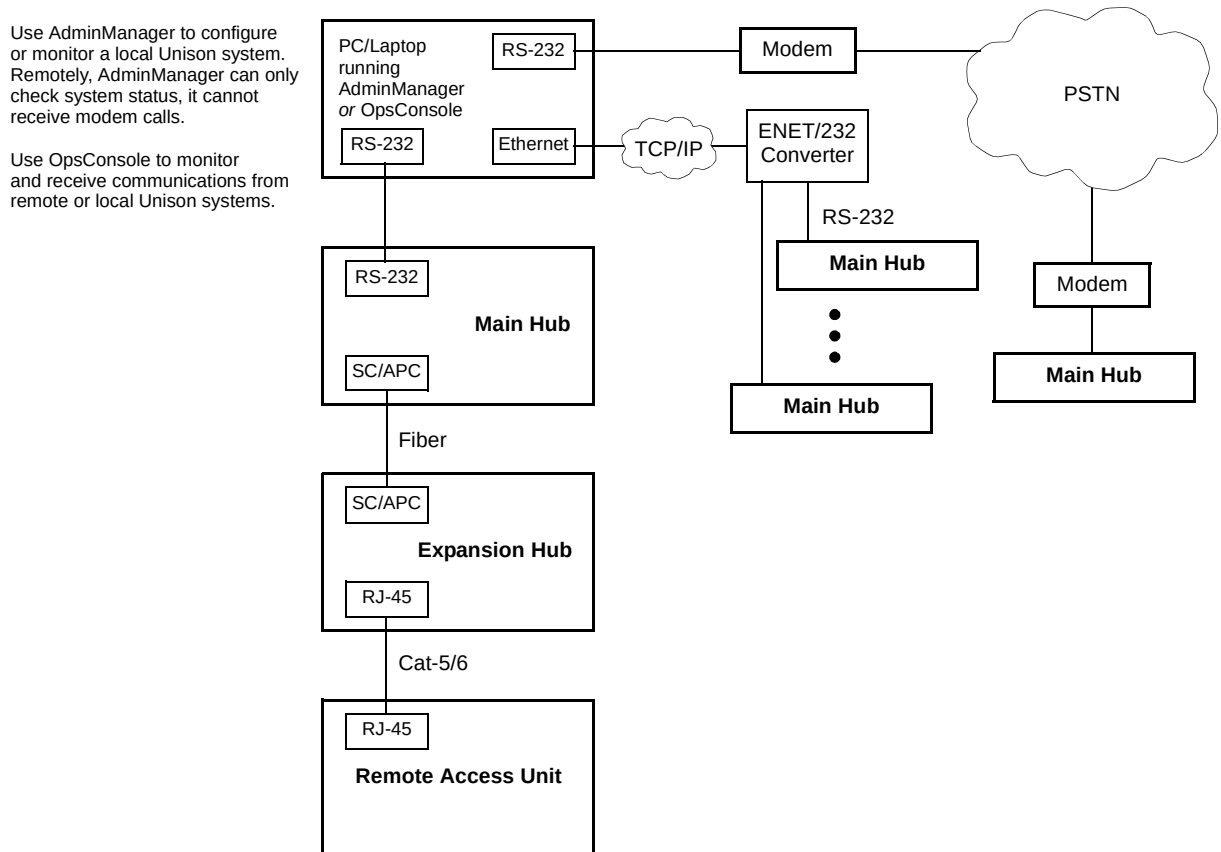
Figure 2-2 OA&M Communications
