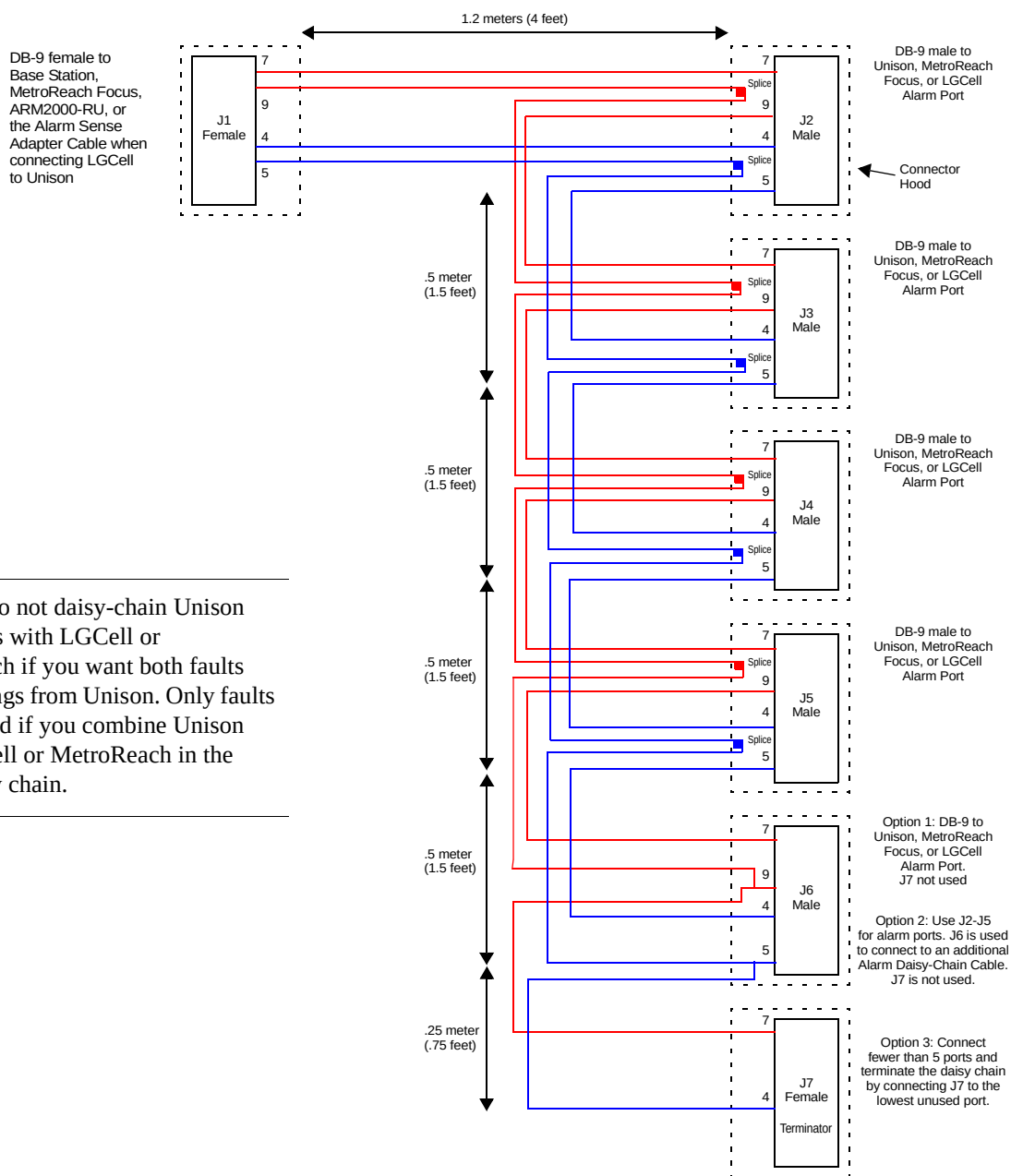
Figure 7-10 5-port Alarm Daisy-Chain Cable
