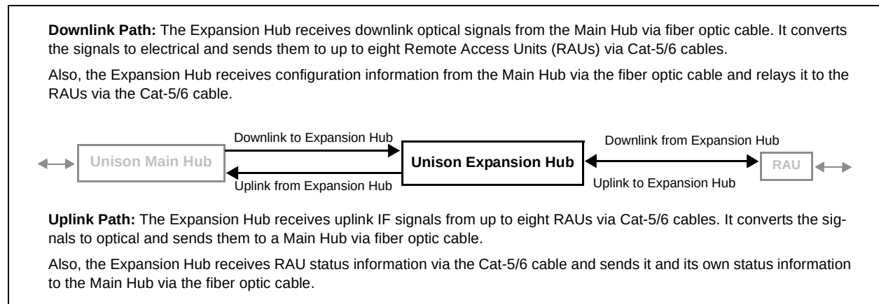
Figure 4-1 Expansion Hub in a Unison System
