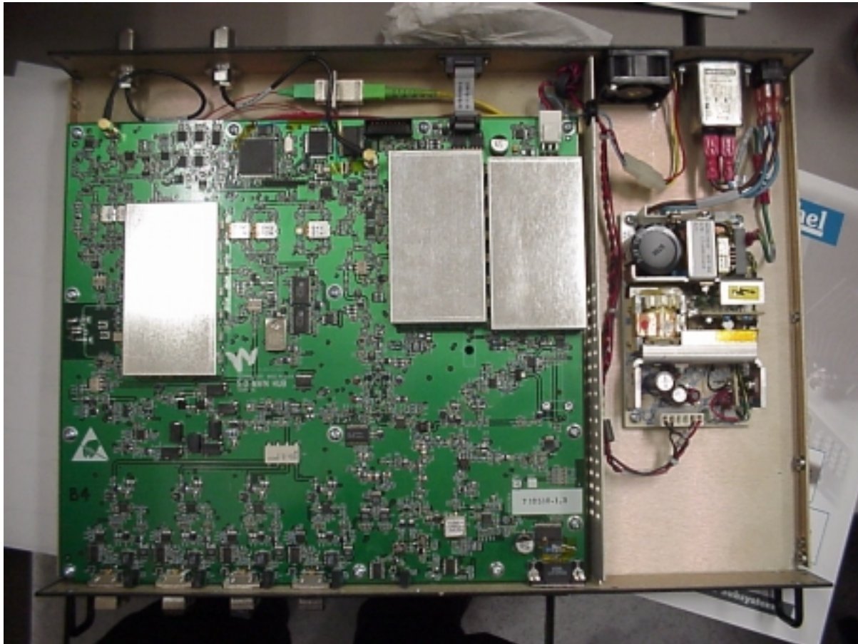
INSIDE OF MAIN HUB (WITH SHIELDS)
