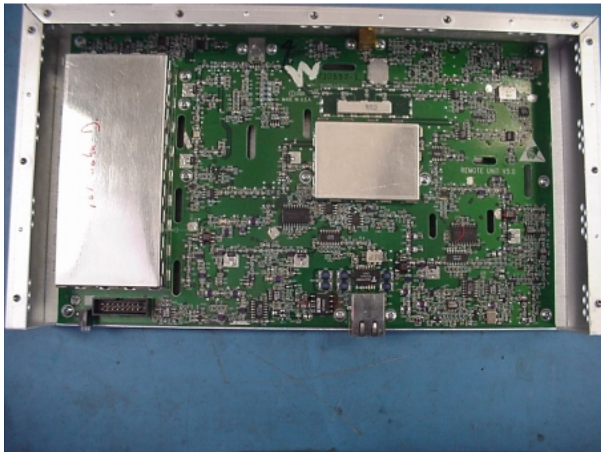
RAU INTERNAL (WITH SHIELDS)
