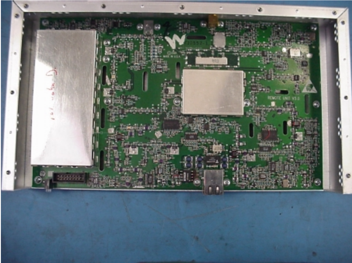
PCS RAU INTERNAL (WITH SHIELDS)
