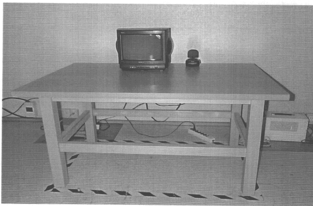
Back View of Conducted Emission Test ( Maximum Testing Configuration)
