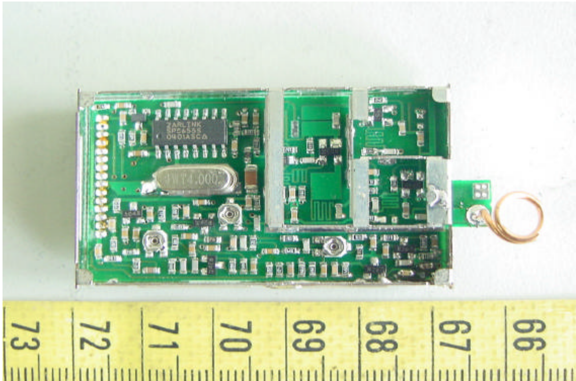
Component View of RF Module's PCB
