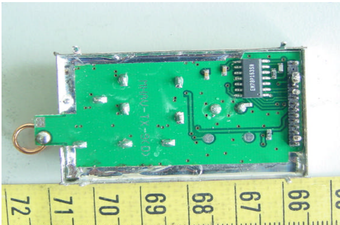
Solder View of RF Module's PCB
