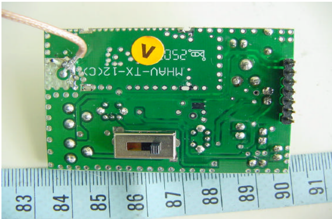
Solder View of Main PCB (Transmitter)
