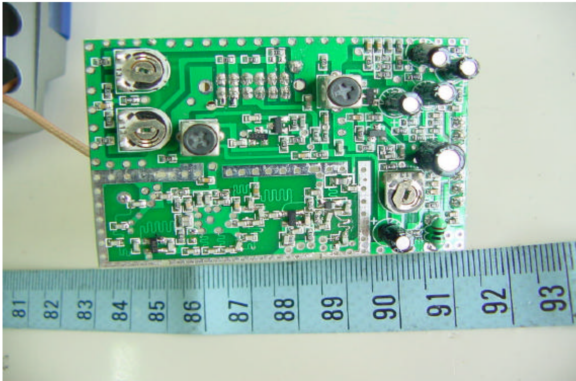
Component View of Main PCB (Transmitter)
