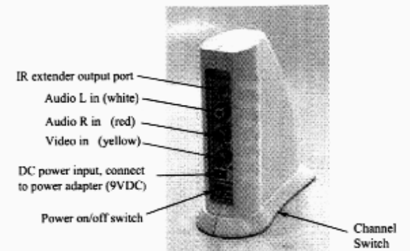
REAR VIEW FOR TRANSMITTER
