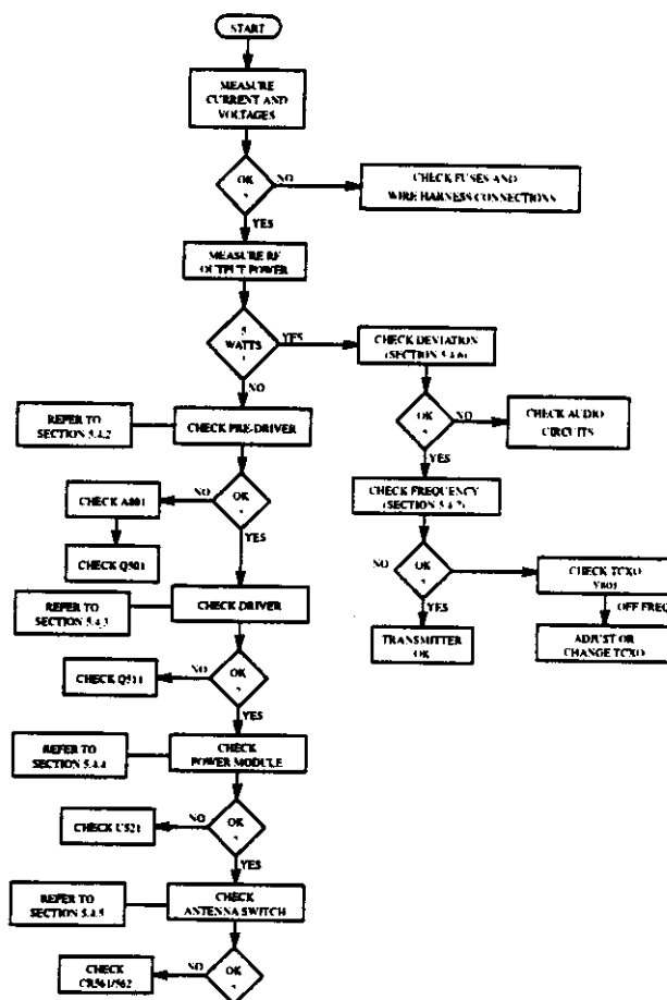
Figure 5-2 TRANSMITTER SERVICING
