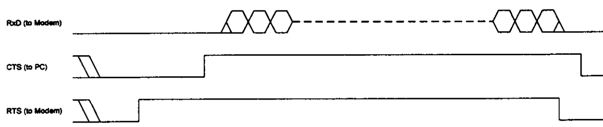
Figure 4-3 RTS/CTS Handshaking Protocol (Resembling a PTT Signal)
