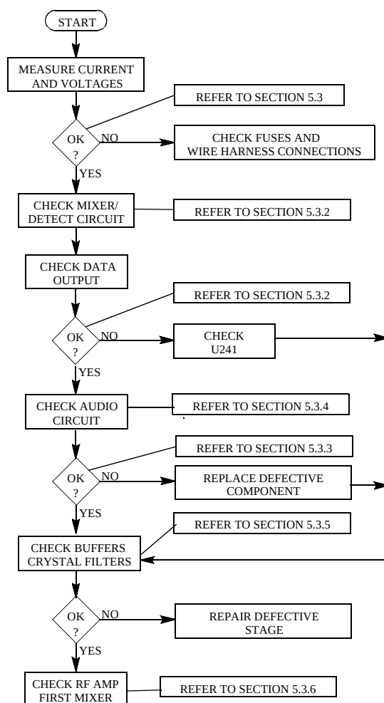
Figure 5-1 RECEIVER SERVICING
