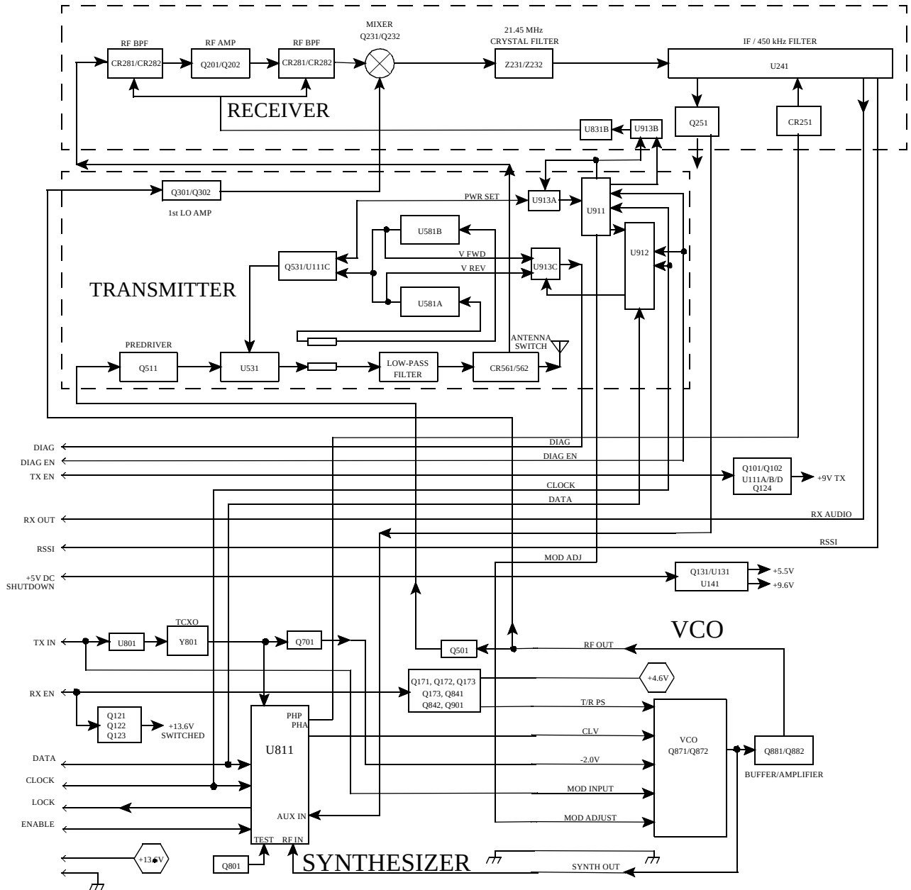
Figure 4-1 Transceiver Block Diagram
