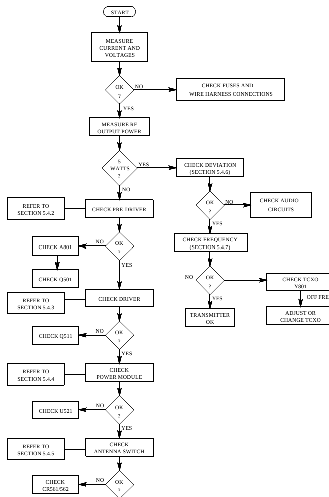
Figure 5-2 TRANSMITTER SERVICING
