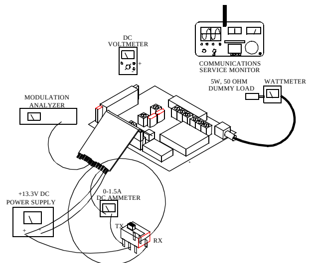
Figure 6-1 TRANSMITTER TEST SETUP
