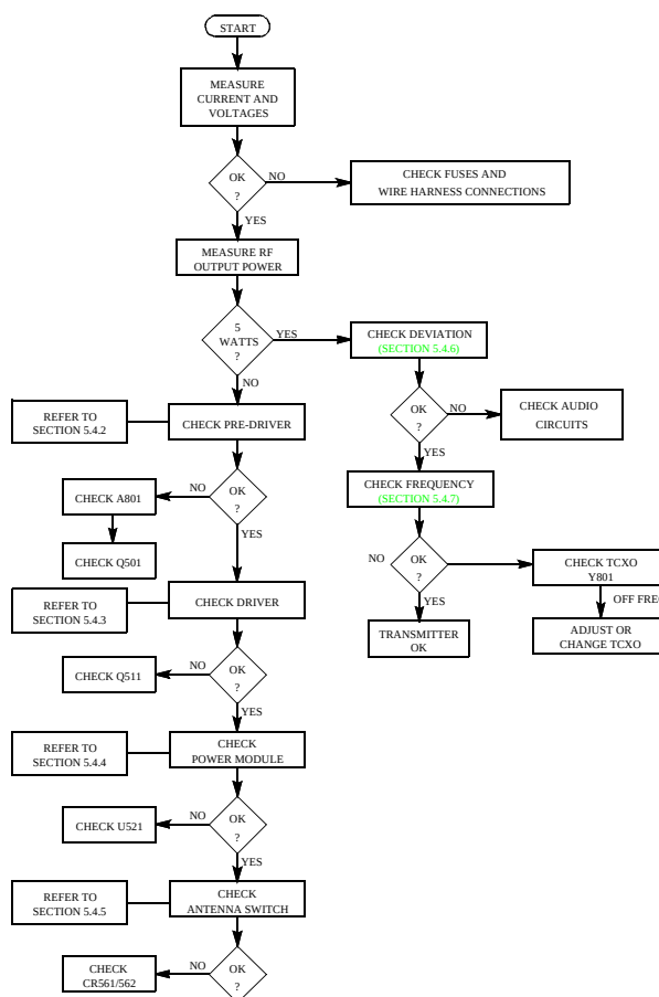
Figure 5-2 TRANSMITTER SERVICING
