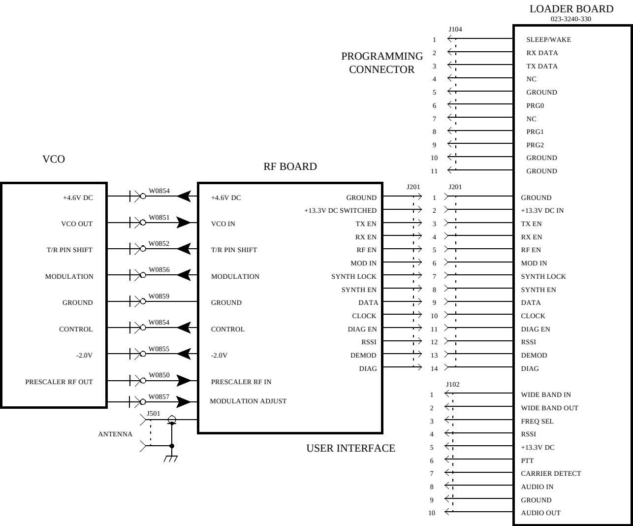
Figure 8-1 3412 INTERCONNECT
