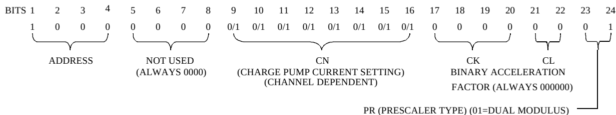
Figure 3-3 B-WORD
