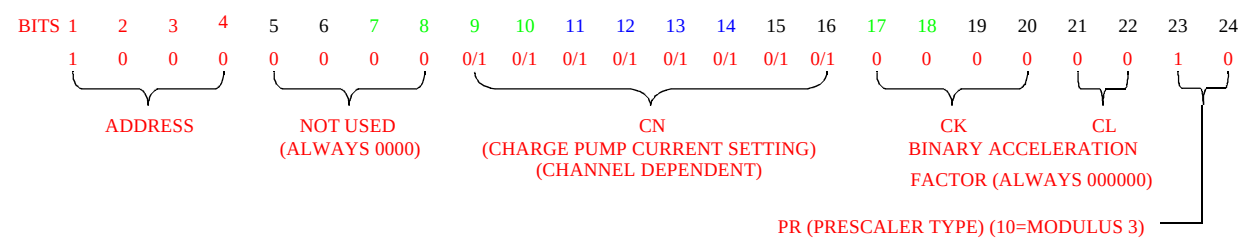
Figure 3-4 B-WORD
