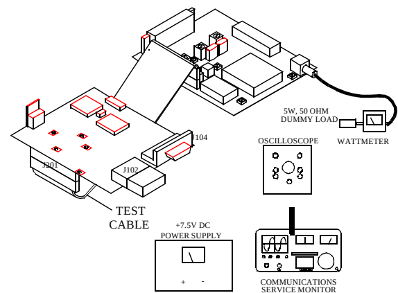
Figure 6-2 TX WITH LOADER TEST SETUP
