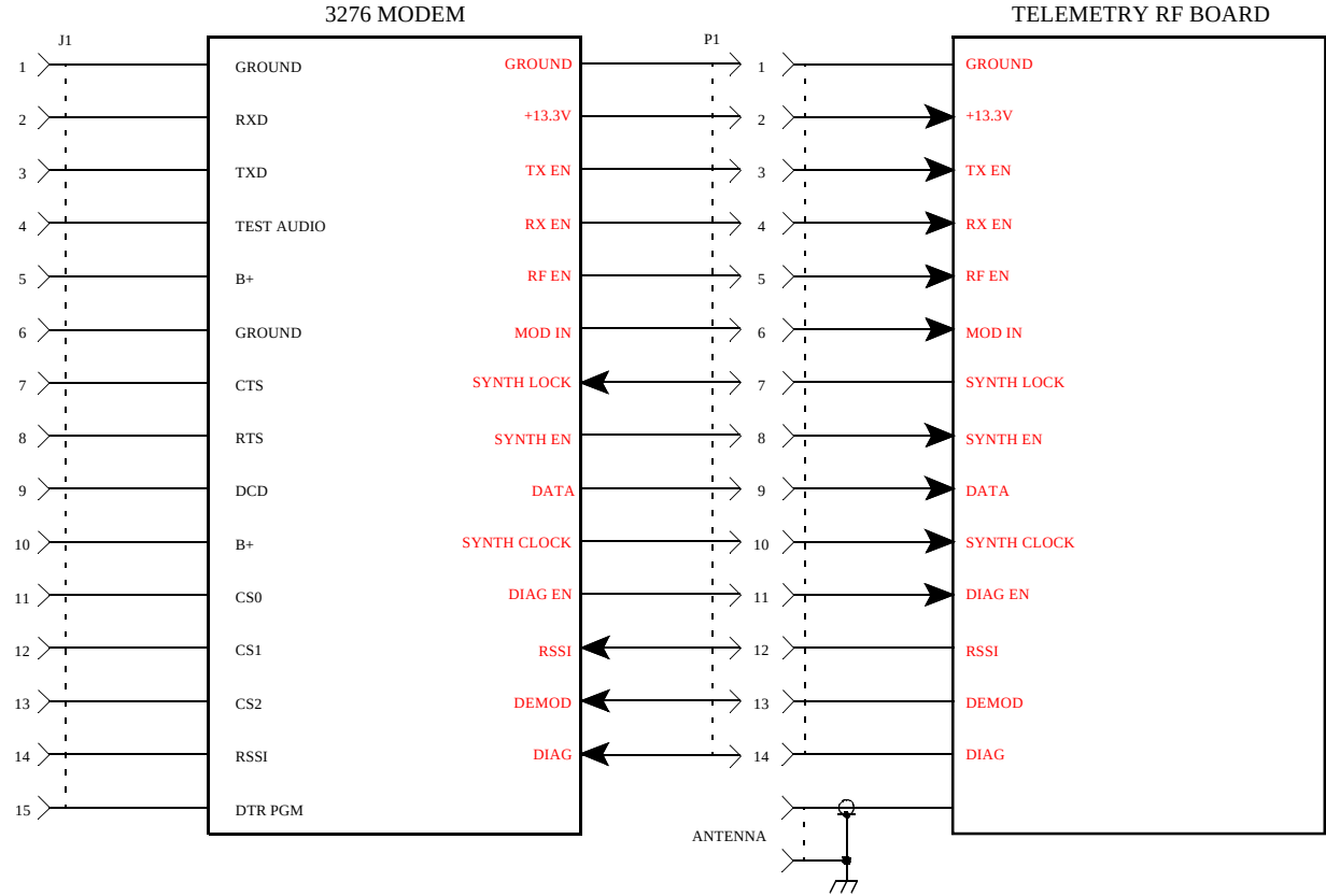
Figure 8-2 MODEM INTERCONNECT
