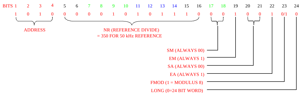
Figure 3-2 D-WORD
