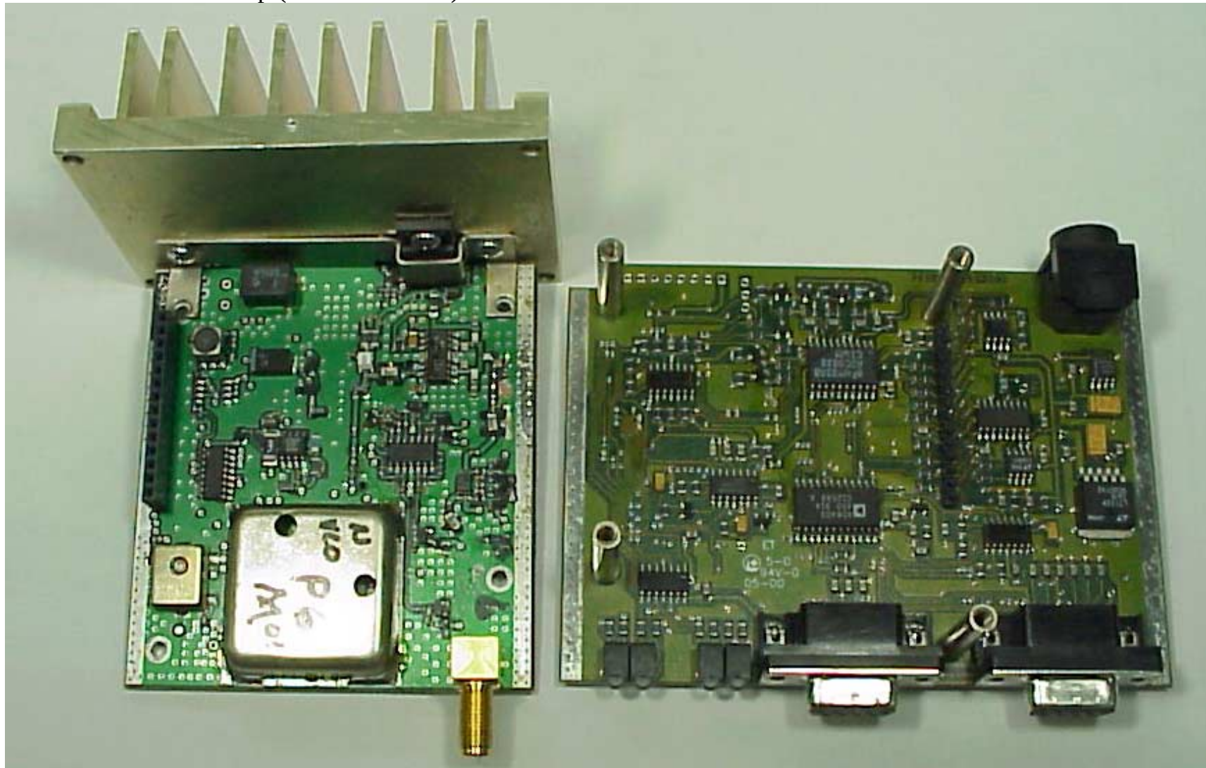
Photo 4: Internal Top (RF and Modem)
