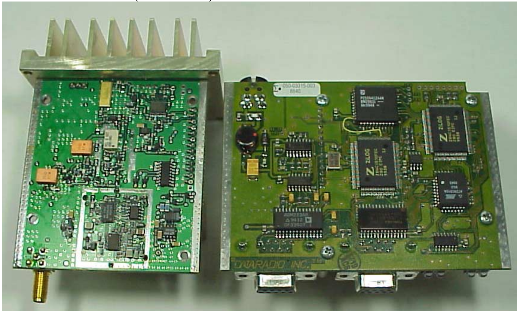
Photo 5: Internal Bottom (RF and Modem)
