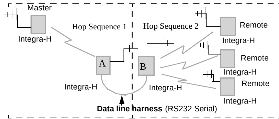
Figure 1-9 Point-Multipoint (Repeater)
